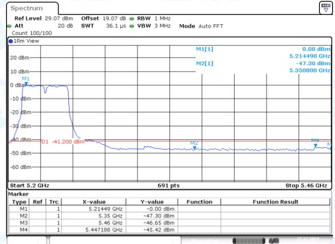
11AC40MIMO-Ant2-5230-PASS
