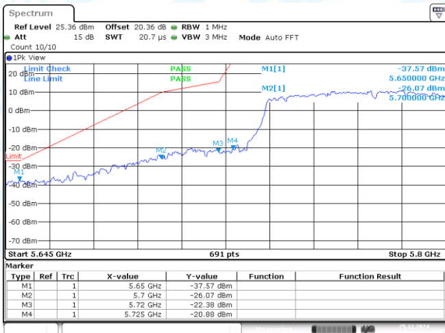
11AC80MIMO-Ant1-5775-PASS
