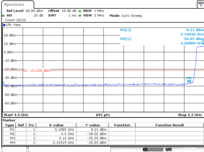
11AC40MIMO-Ant1-5190-PASS
