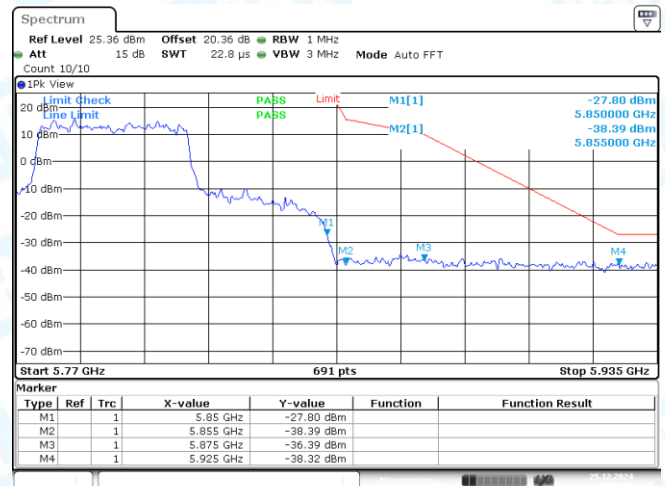
11AX40MIMO-Ant2-5755-PASS
