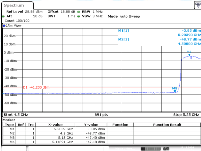
11AC80MIMO-Ant2-5210-PASS
