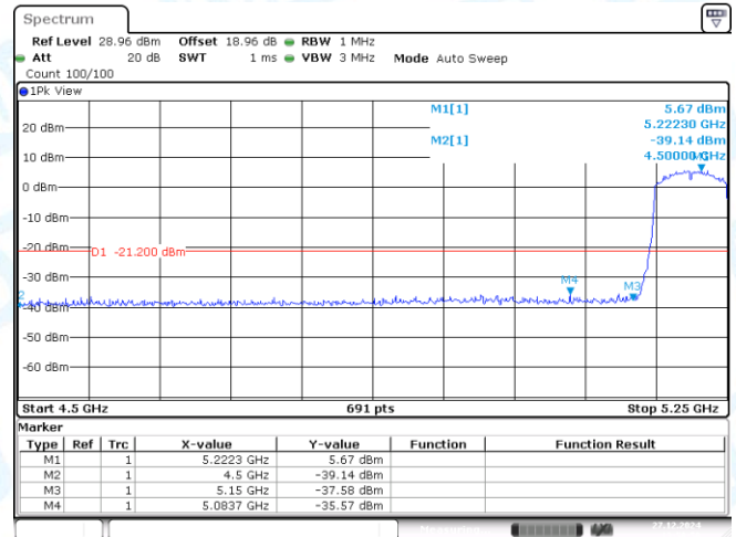
11AC80MIMO-Ant1-5210-PASS
