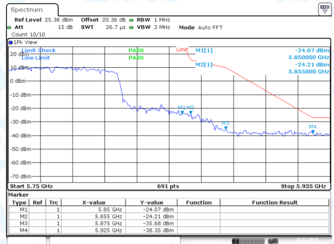
11AC80MIMO-Ant1-5775-PASS
