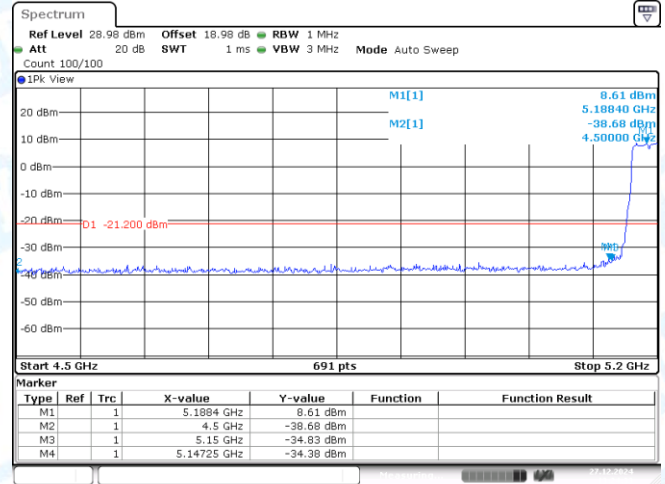
11AC40MIMO-Ant2-5190-PASS
