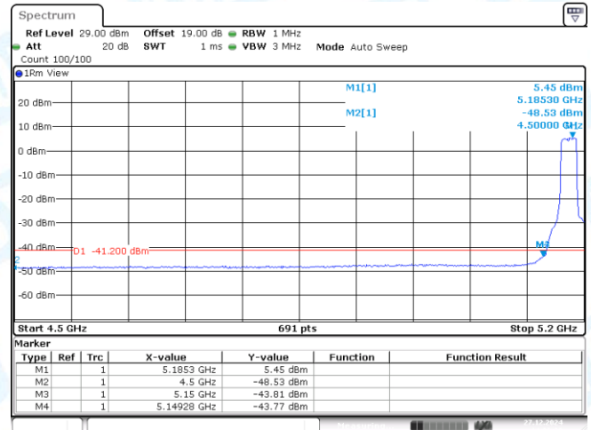
11AX20MIMO-Ant2-5180-PASS
