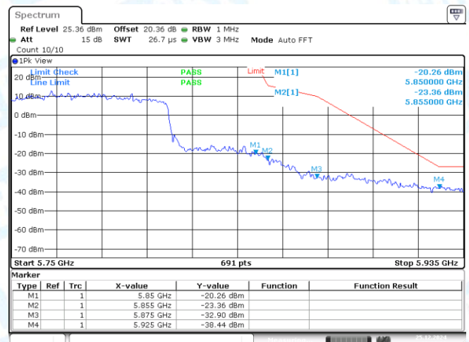
11AX80MIMO-Ant1-5775-PASS
