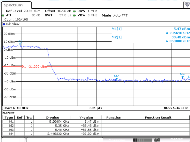
11AC80MIMO-Ant1-5210-PASS
