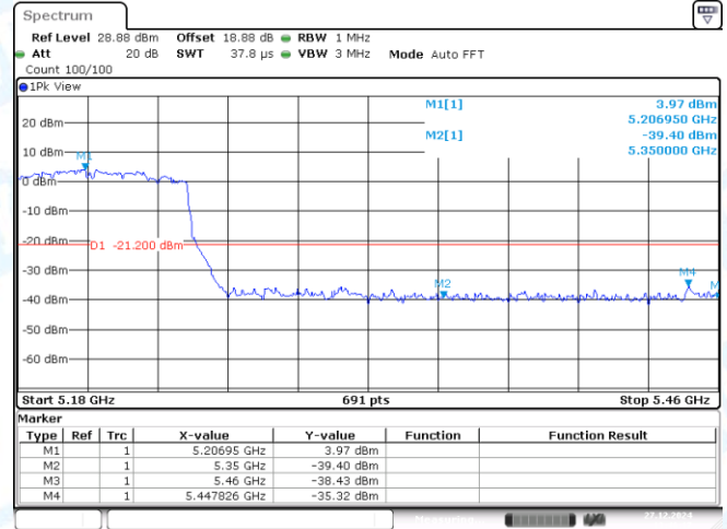
11AC80MIMO-Ant1-5210-PASS
