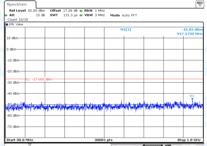
11AX80MIMO-Ant2-5775-30~1000-PASS
