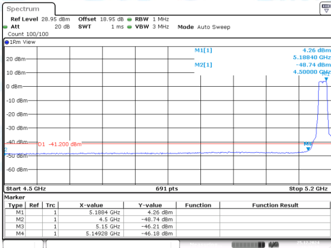
11N20MIMO-Ant1-5180-PASS
