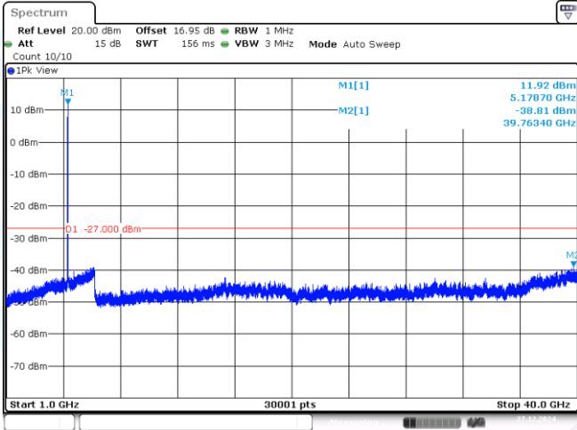
11AX20MIMO-Ant1-5180-1000~40000-PASS
