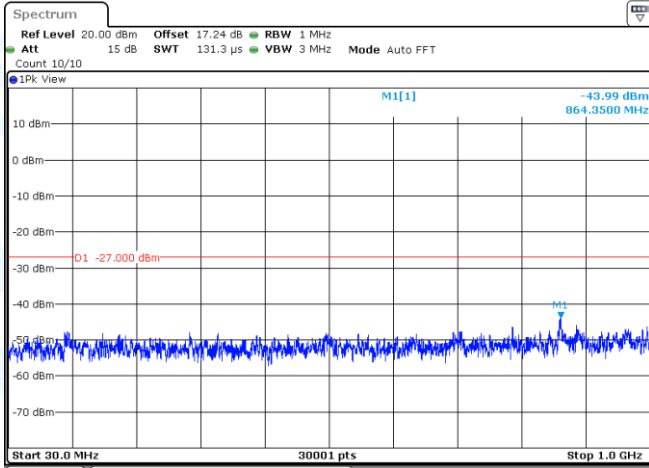
11AX20MIMO-Ant1-5825-30~1000-PASS
