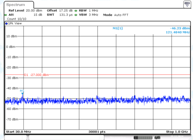
11AC40MIMO-Ant2-5755-30~1000-PASS
