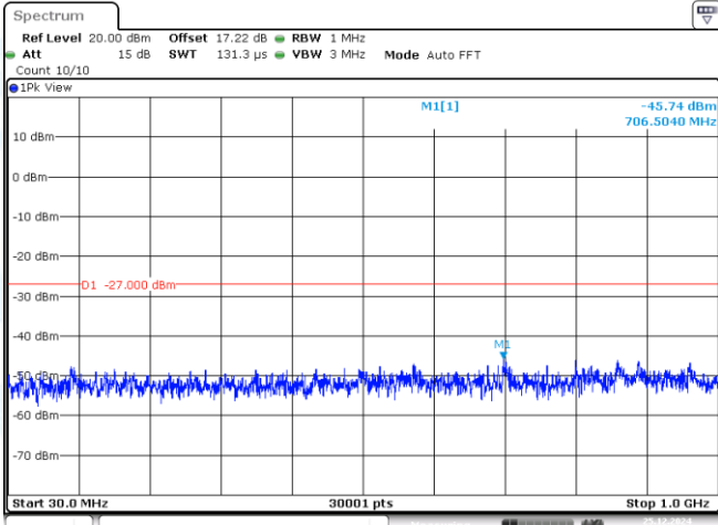
11AX80MIMO-Ant1-5775-30~1000-PASS
