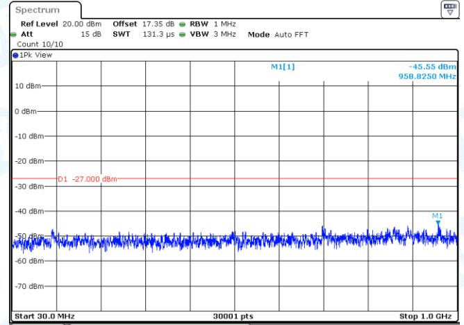
11AX20MIMO-Ant2-5825-30~1000-PASS
