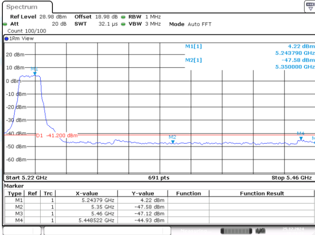
11A-CDD-Ant1-5240-PASS
