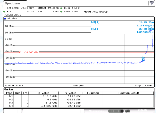
11N20MIMO-Ant2-5180-PASS
