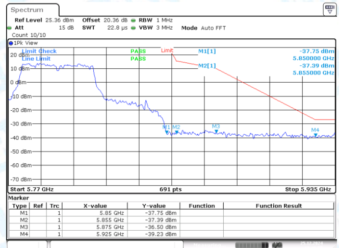
11N40MIMO-Ant2-5755-PASS
