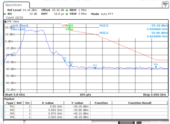
11A-CDD-Ant2-5745-PASS
