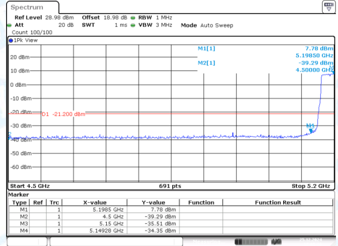
11N40MIMO-Ant2-5190-PASS
