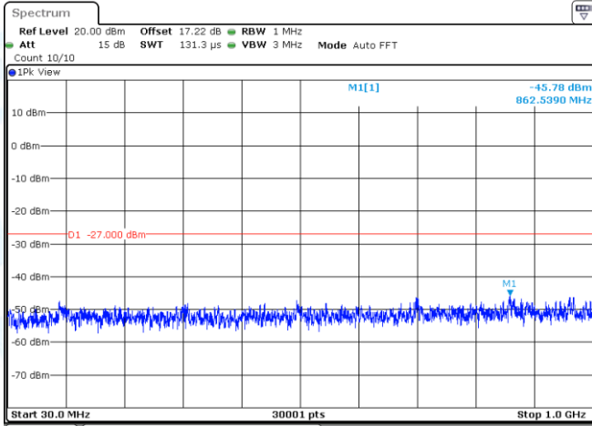
11AC80MIMO-Ant1-5775-30~1000-PASS
