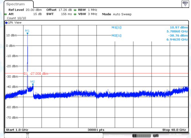
11AC40MIMO-Ant2-5795-1000~40000-PASS
