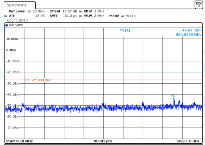
11AX20MIMO-Ant2-5240-30~1000-PASS
