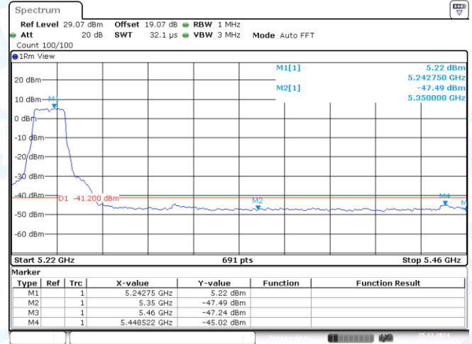
11A-CDD-Ant2-5240-PASS
