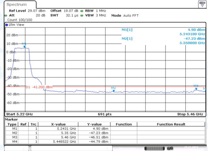
11N20MIMO-Ant2-5240-PASS
