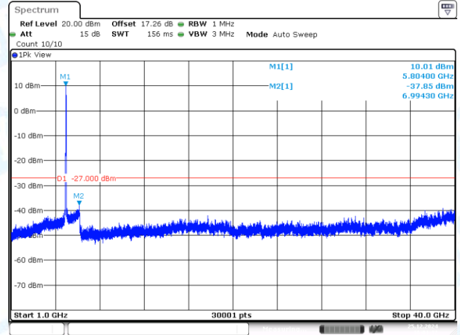
11AX40MIMO-Ant2-5795-1000~40000-PASS
