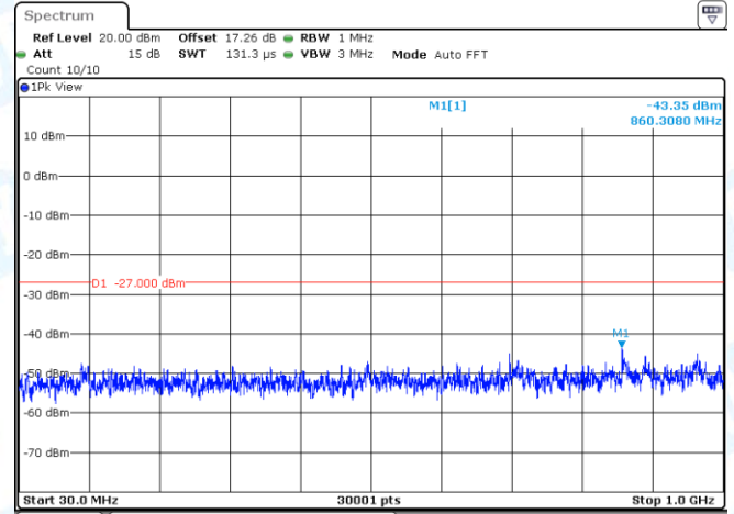
11AC80MIMO-Ant2-5775-30~1000-PASS
