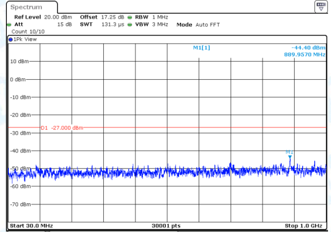
11AX40MIMO-Ant2-5755-30~1000-PASS
