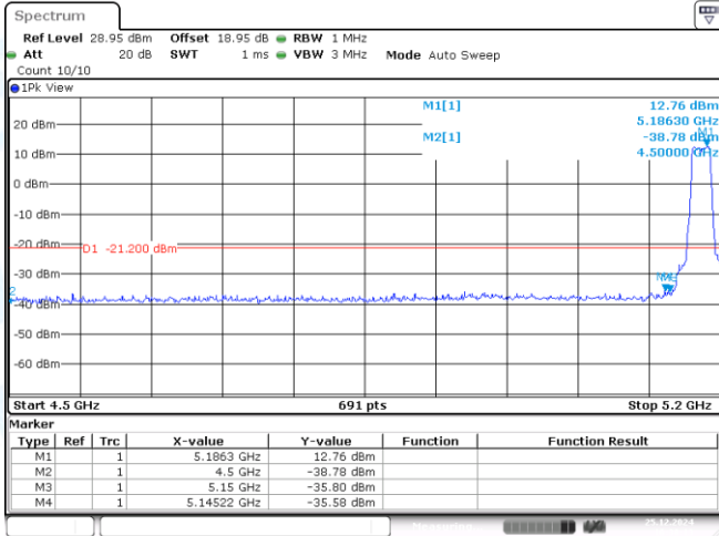
11N20MIMO-Ant1-5180-PASS
