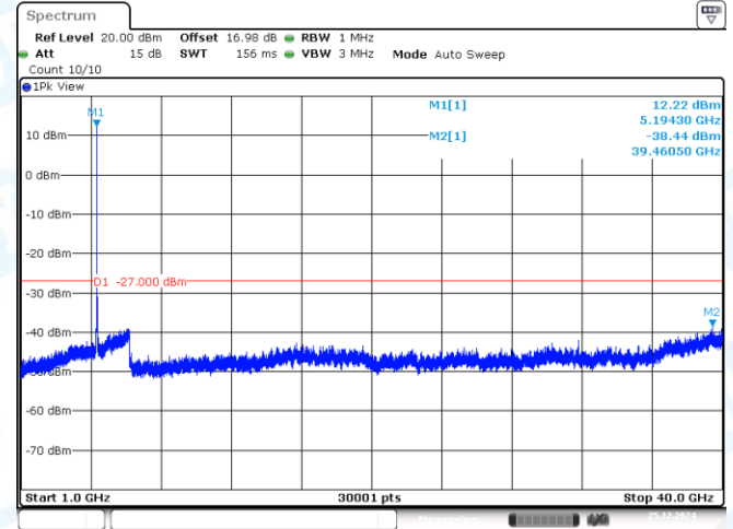
11A-CDD-Ant2-5200-1000~40000-PASS
