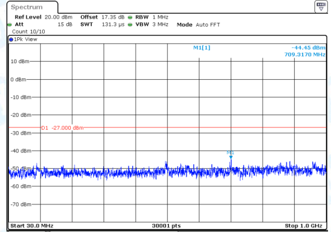
11AC20MIMO-Ant2-5825-30~1000-PASS
