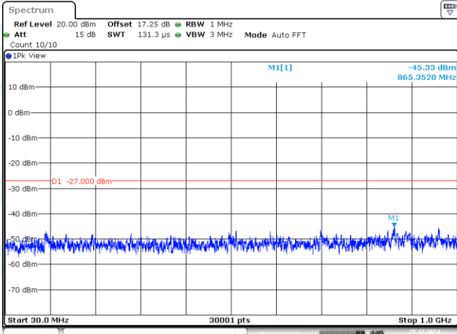
11A-CDD-Ant1-5745-30~1000-PASS
