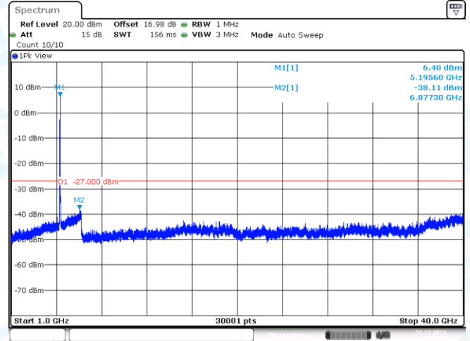
11AC40MIMO-Ant2-5190-1000~40000-PASS
