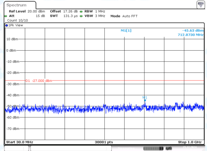
11N40MIMO-Ant2-5795-30~1000-PASS
