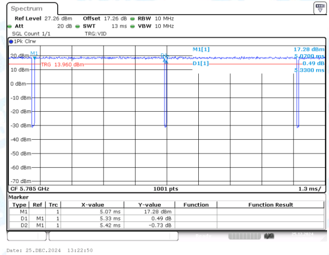
NTNV-11N20MIMO-Ant2-5785
