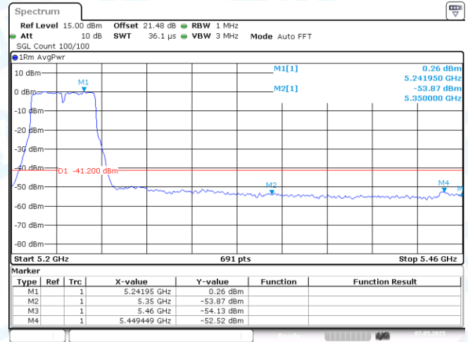
11AC40MIMO-Ant2-5230-PASS
