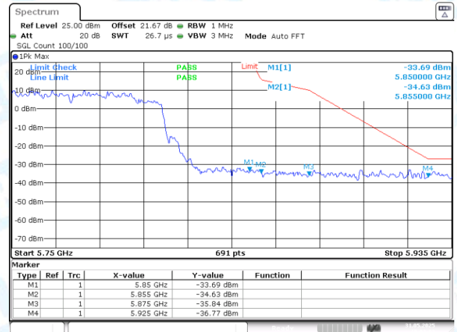
11AC80MIMO-Ant1-5775-PASS
