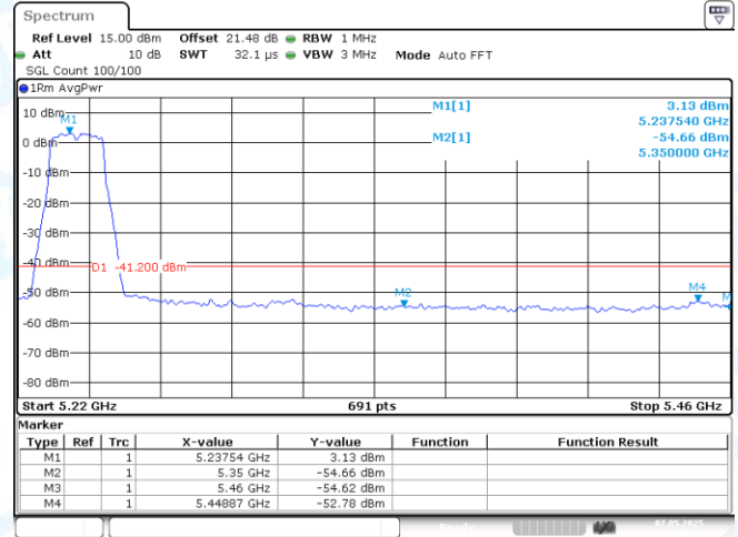
11AC20MIMO-Ant2-5240-PASS
