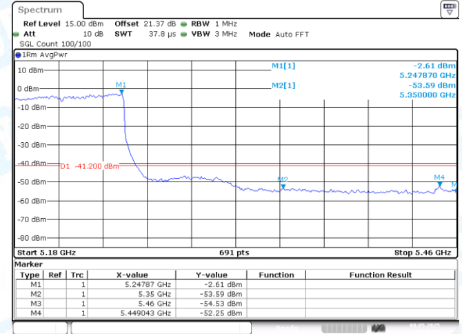
11AX80MIMO-Ant2-5210-PASS
