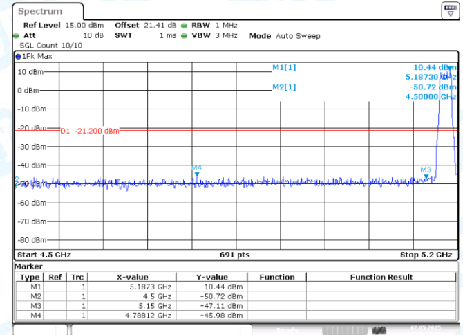
11AC20MIMO-Ant2-5180-PASS
