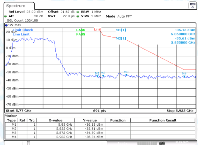
11AC40MIMO-Ant2-5755-PASS
