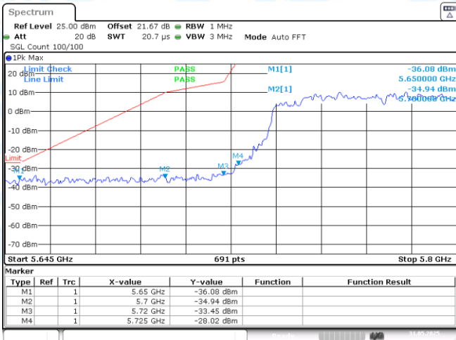
11AC80MIMO-Ant1-5775-PASS
