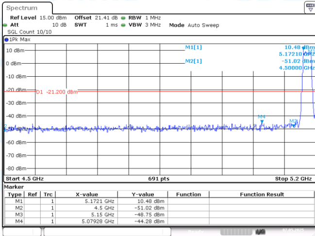
11N20MIMO-Ant2-5180-PASS
