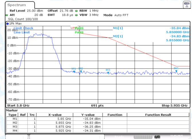
11N20MIMO-Ant2-5745-PASS
