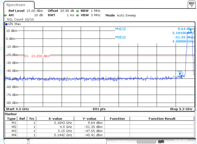
11N20MIMO-Ant1-5180-PASS
