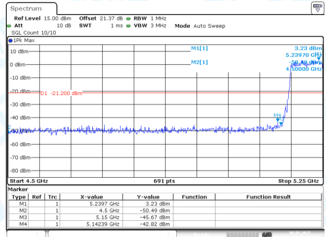
11AC80MIMO-Ant2-5210-PASS
