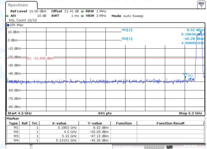
11AX20MIMO-Ant2-5180-PASS
