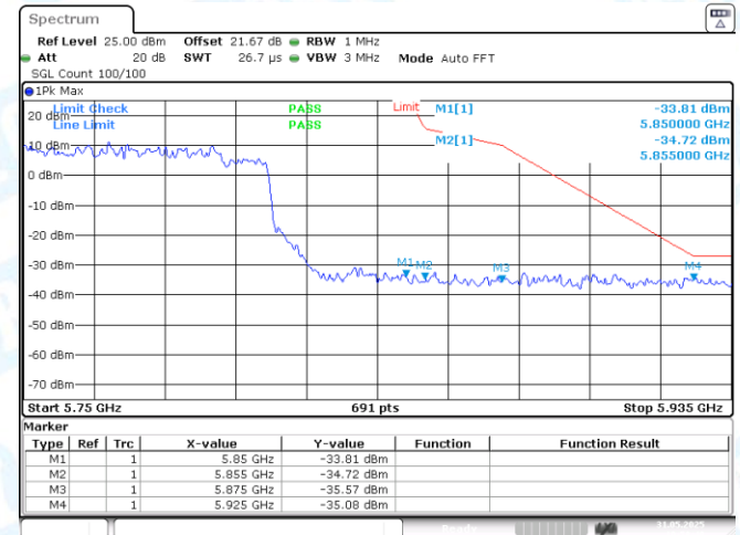
11AX80MIMO-Ant1-5775-PASS
