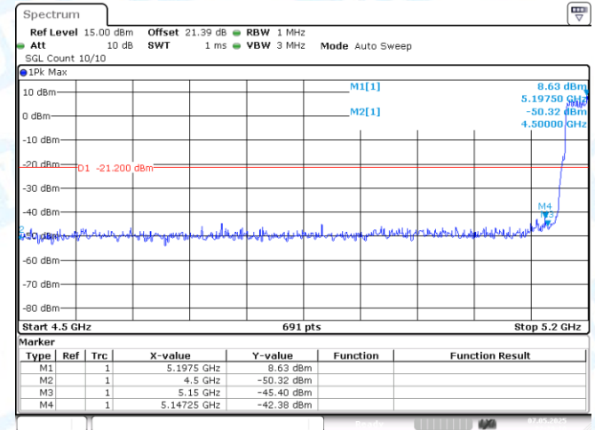
11N40MIMO-Ant2-5190-PASS
