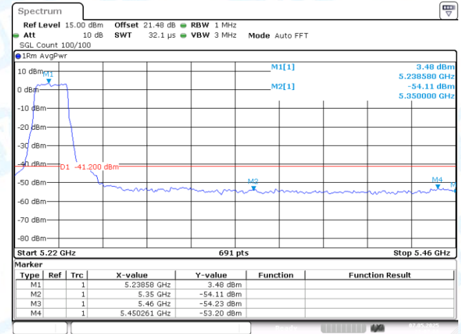
11N20MIMO-Ant2-5240-PASS
