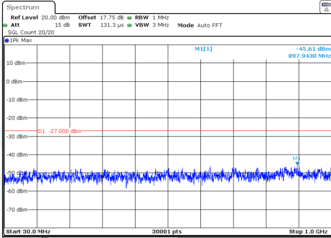
11AC40MIMO-Ant1-5755-30~1000-PASS
