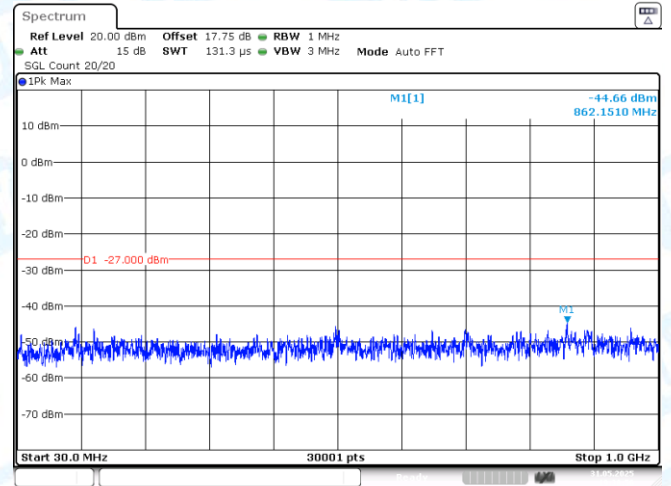
11AX40MIMO-Ant2-5755-30~1000-PASS
