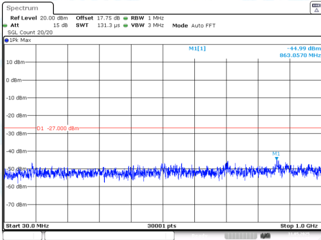
11AX40MIMO-Ant1-5755-30~1000-PASS
