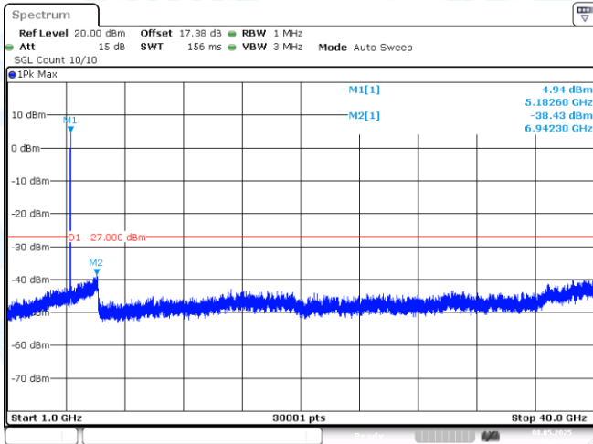
11AX40MIMO-Ant1-5190-1000~40000-PASS
