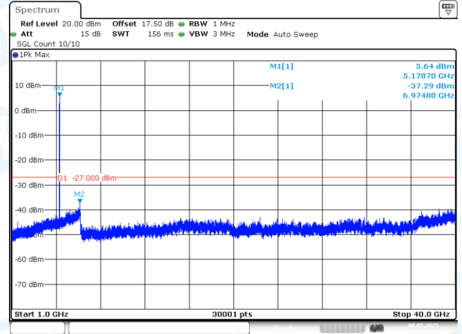
11AX20MIMO-Ant2-5180-1000~40000-PASS
