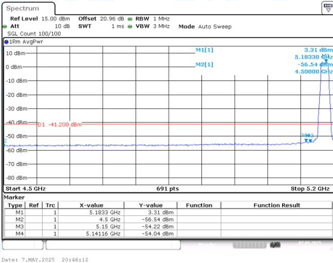
11A-CDD-Ant1-5180-PASS
