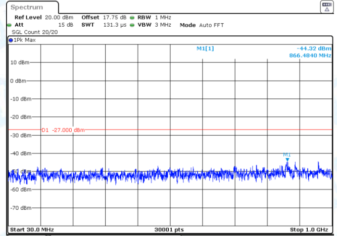
11AC40MIMO-Ant2-5755-30~1000-PASS
