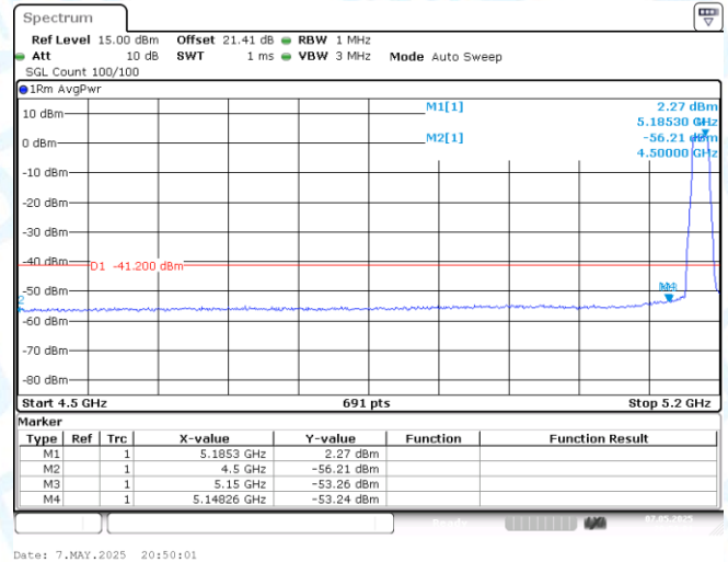
11A-CDD-Ant2-5180-PASS
