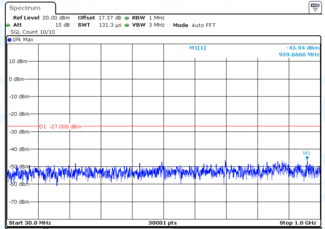
11AX20MIMO-Ant2-5240-30~1000-PASS
