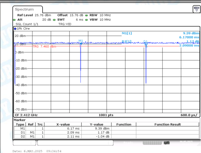
NTNV-11G-CDD-Ant2-2412
