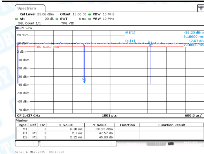
NTNV-11G-CDD-Ant1-2437
