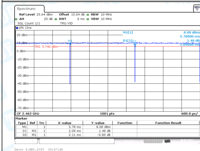
NTNV-11G-CDD-Ant1-2462
