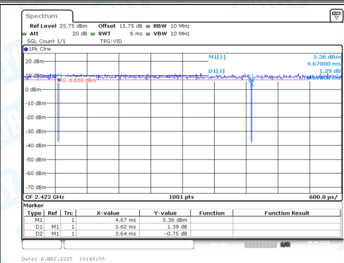
NTNV-11AX40MIMO-Ant2-2422
