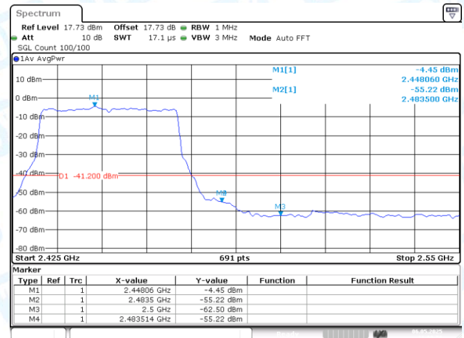
11AX40MIMO-Ant2-2452-PASS
