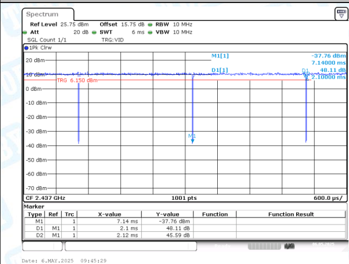
NTNV-11G-CDD-Ant2-2437
