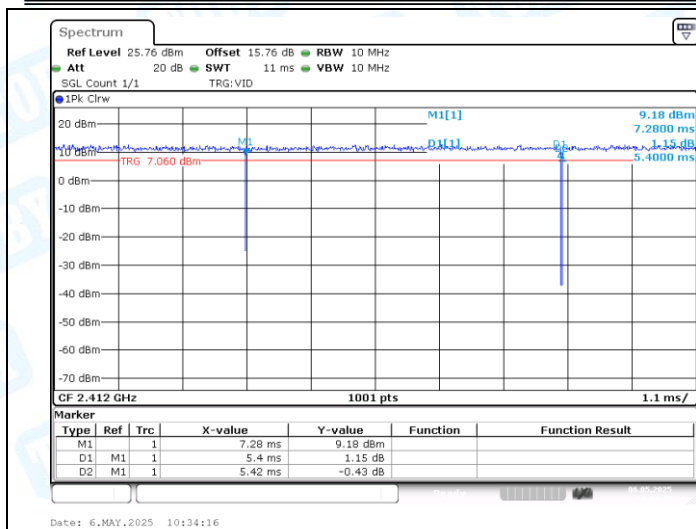
NTNV-11AX20MIMO-Ant2-2412
