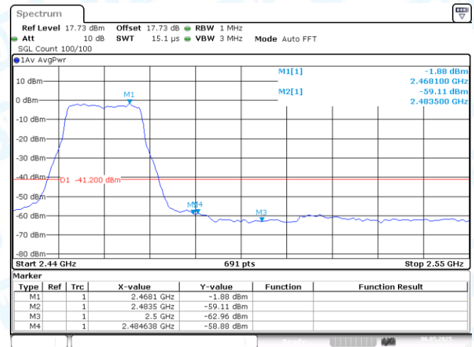
11N20MIMO-Ant2-2462-PASS
