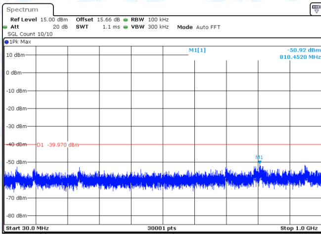
11AX40MIMO-Ant1-2422-0~Reference-PASS
