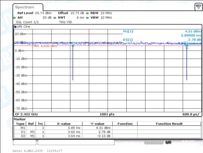
NTNV-11AX40MIMO-Ant2-2452
