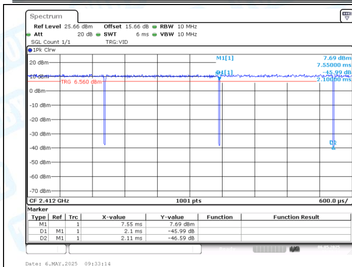
NTNV-11G-CDD-Ant1-2412
