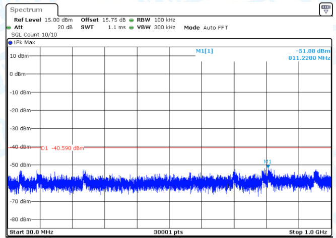
11AX40MIMO-Ant2-2422-0~Reference-PASS
