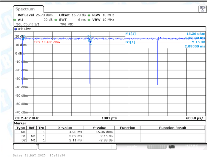
NTNV-11AX20MIMO-Ant2-2462
