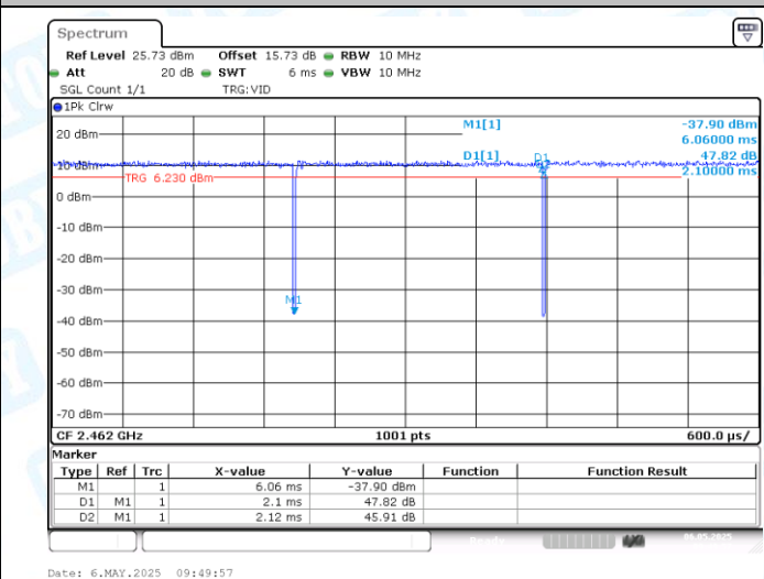
NTNV-11G-CDD-Ant2-2462
