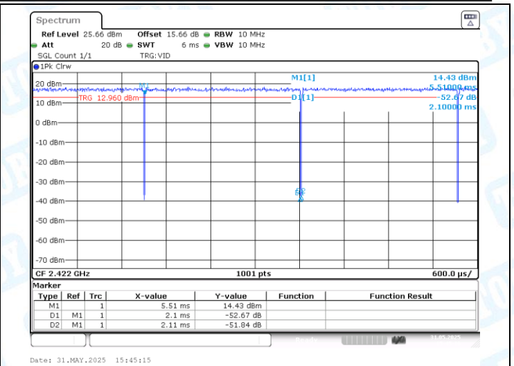
NTNV-11N40MIMO-Ant1-2422
