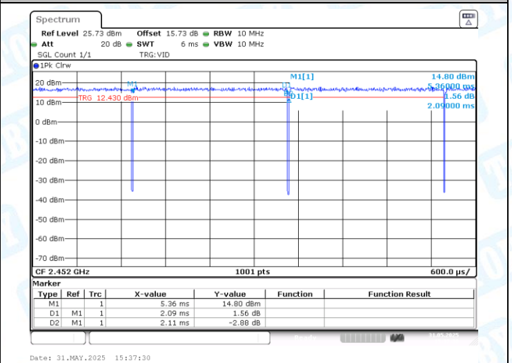
NTNV-11N40MIMO-Ant2-2452
