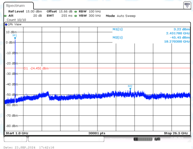
11N20SISO-Ant1-2437-1000~26500-PASS
