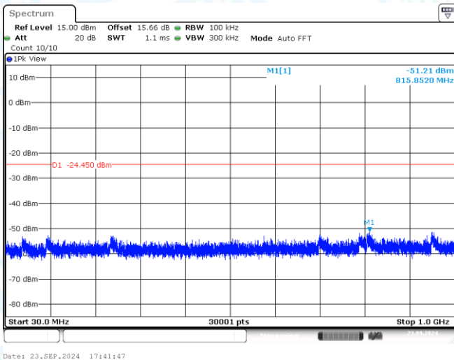
11N20SISO-Ant1-2437-30~1000-PASS
