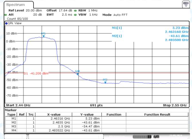
11G-Ant1-2462-PASS
