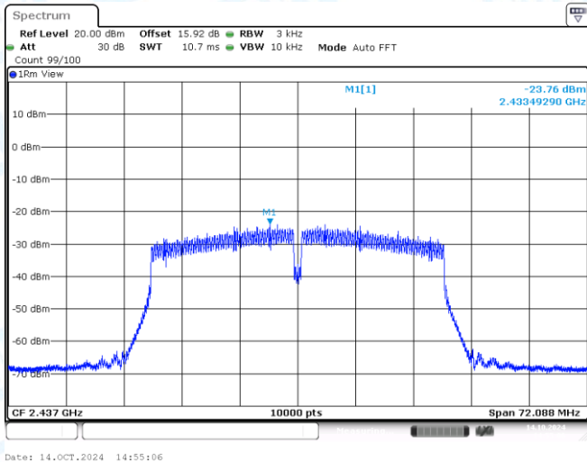
11N40SISO-Ant1-2437-PASS
