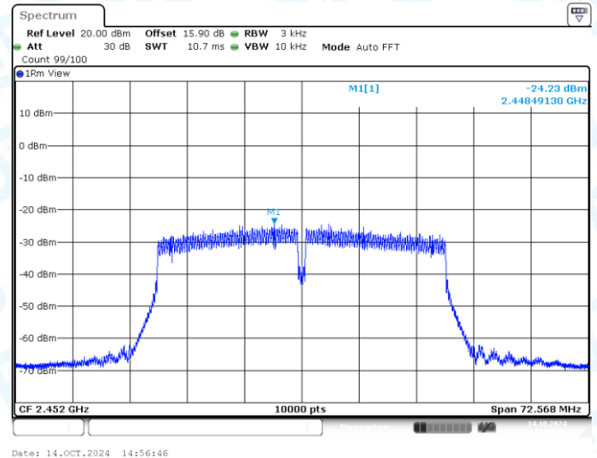
11N40SISO-Ant1-2452-PASS
