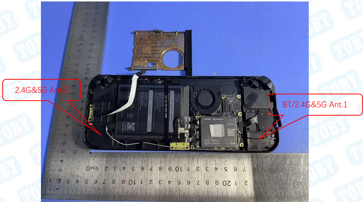
Photo 8 Internal of EUT
