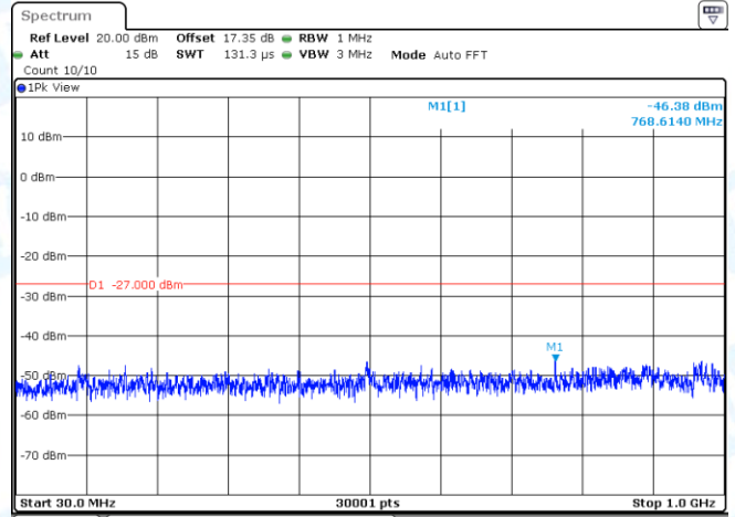
11AX20MIMO-Ant2-5825-30~1000-PASS
