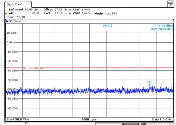
11AX40MIMO-Ant2-5755-30~1000-PASS
