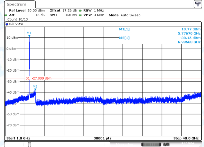
11AX40MIMO-Ant2-5795-1000~40000-PASS
