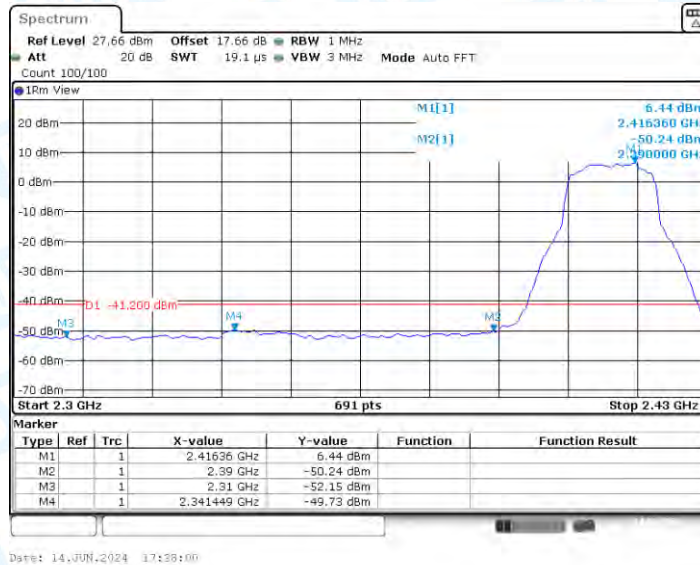
11G-CDD_Ant1_Low_2412_Peak
