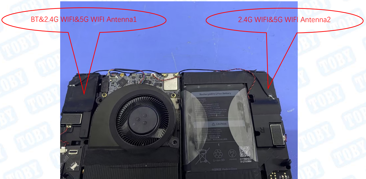
Photo 13 Internal of EUT
