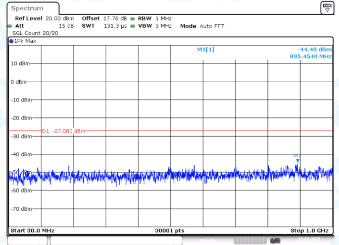
11AC80MIMO-Ant2-5775-30~1000-PASS
