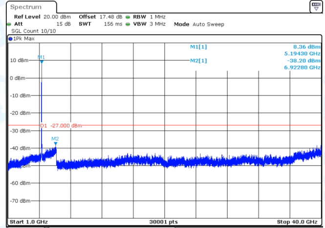
11AX40MIMO-Ant2-5190-1000~40000-PASS
