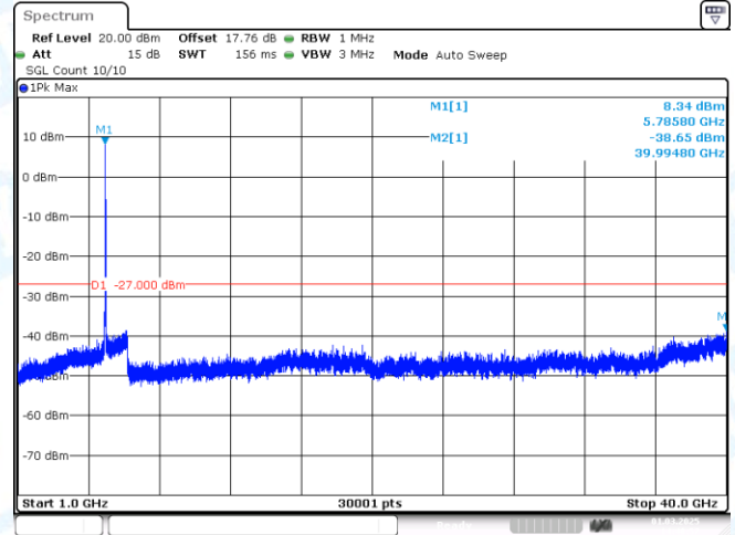
11AC40MIMO-Ant2-5795-1000~40000-PASS
