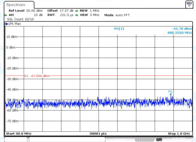
11AC20MIMO-Ant2-5240-30~1000-PASS
