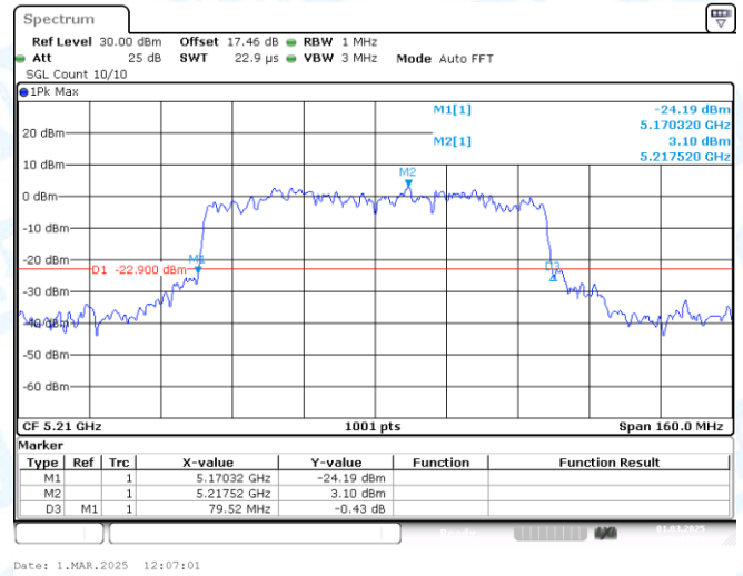
11AC80MIMO-Ant2-5210
