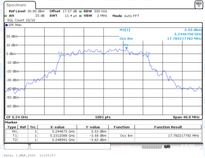
11AC20MIMO-Ant2-5240
