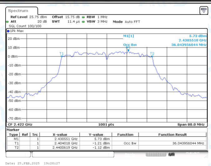
11N40MIMO-Ant2-2422
