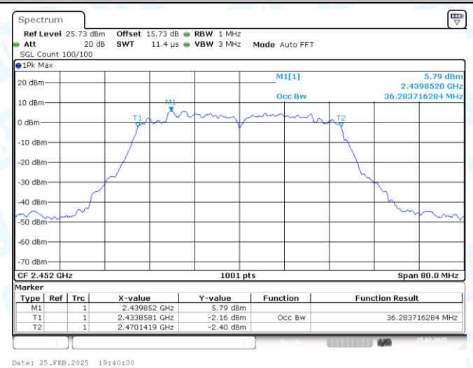
11N40MIMO-Ant2-2452
