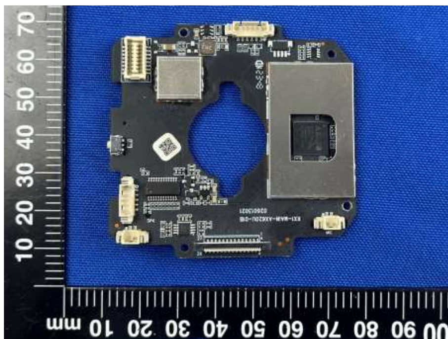
SECONDARY BOARD 3 REAR VIEW (WITH SHIELDING)
