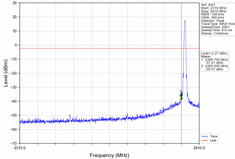
GFSK_DH5_LCH_2402MHz_Ant1_NTNV
