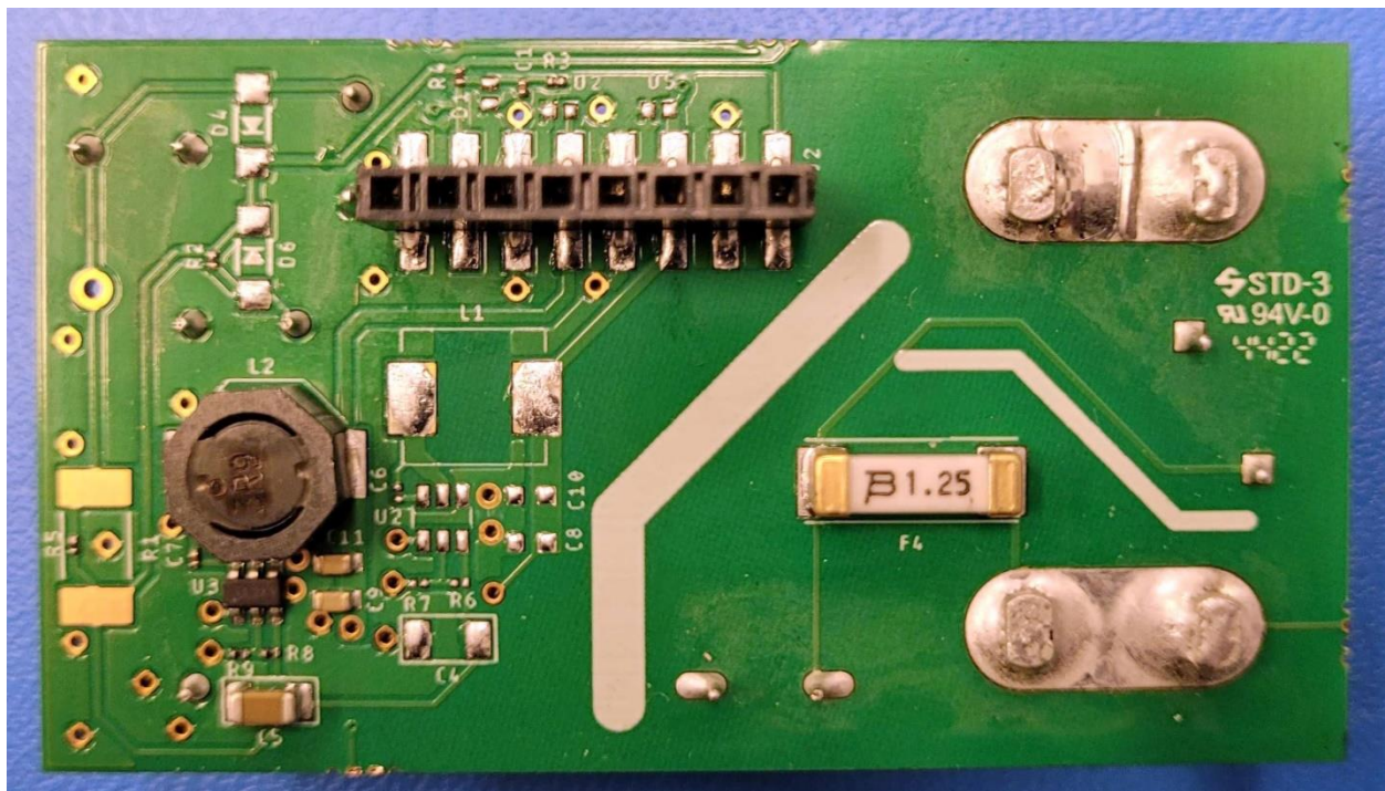
HVB bottom view
