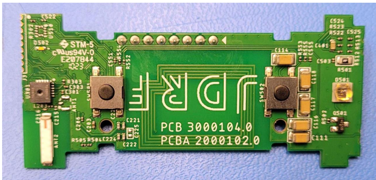
LVB top view
