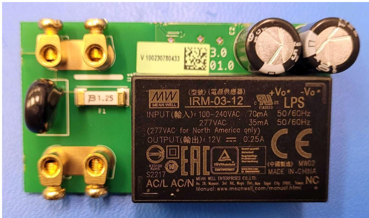
HVB top view
