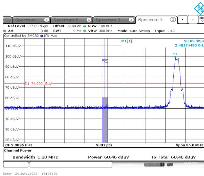
Figure 7.7-10: Band edge spurious emissions at 2390 MHz Peak
