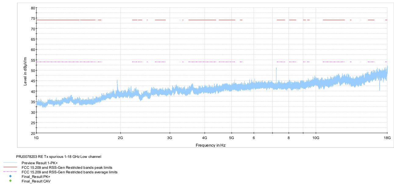
Figure 7.7-4: Radiated spurious emissions 1-18 GHz low channel
