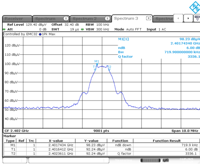
Figure 7.5-1: 6 dB bandwidth on low ch.
