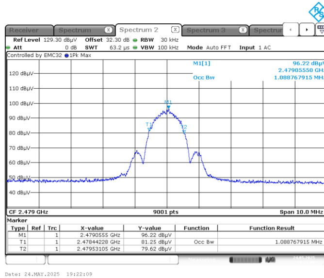
Figure 7.5-6: 99% occupied bandwidth on high ch.
