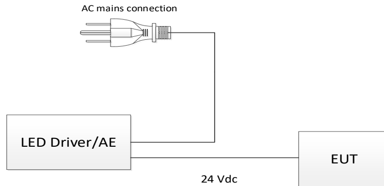
Figure 4.5-1: Radiated testing block diagram
