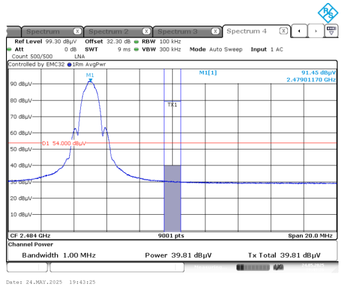
Figure 7.7-13: Band edge spurious emissions at 2483.5 MHz Average
