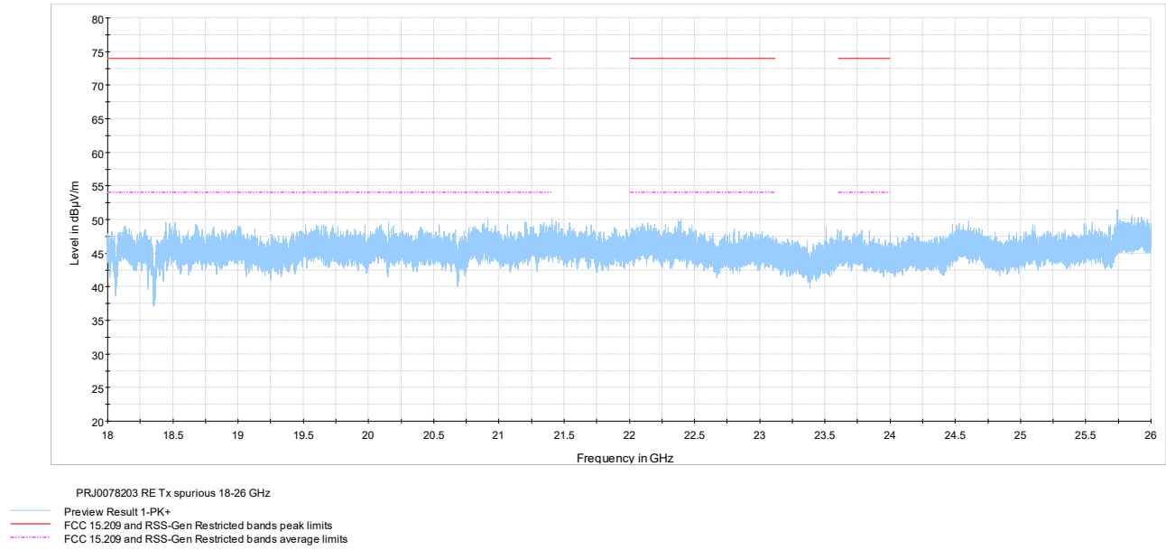
Figure 7.7-7: Radiated spurious emissions 18-26 GHz low channel
