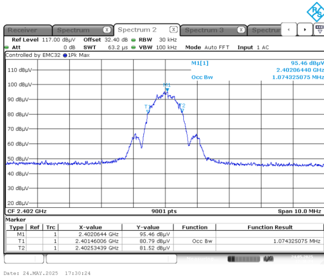
Figure 7.5-4: 99% occupied bandwidth on low ch.
