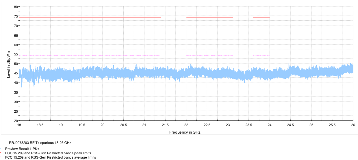
Figure 7.7-9: Radiated spurious emissions 18-26 GHz high channel
