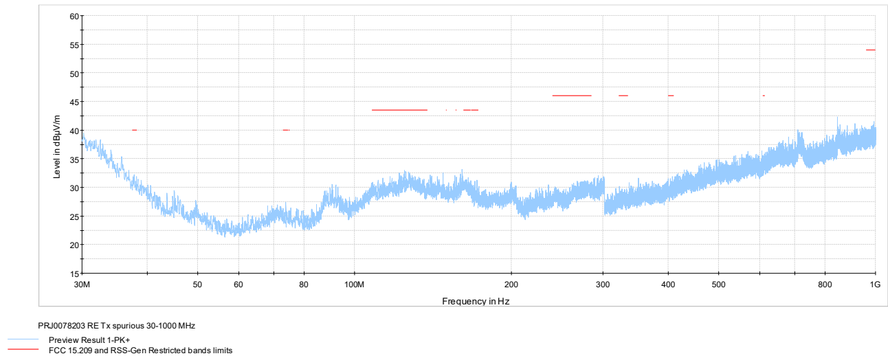
Figure 7.7-3: Radiated spurious emissions 30-1000 MHz high channel
