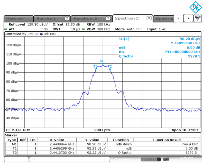
Figure 7.5-2: 6 dB bandwidth on mid ch.
