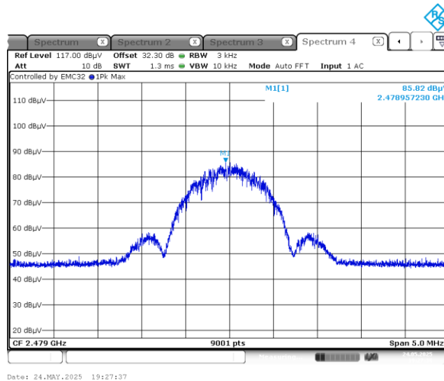
Figure 7.8-3: PSD on high channel
