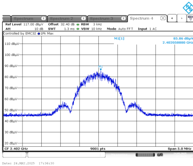
Figure 7.8-1: PSD on low channel
