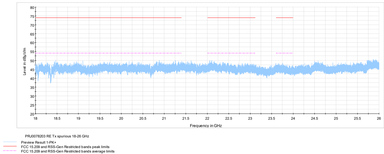
Figure 7.7-8: Radiated spurious emissions 18-26 GHz mid channel
