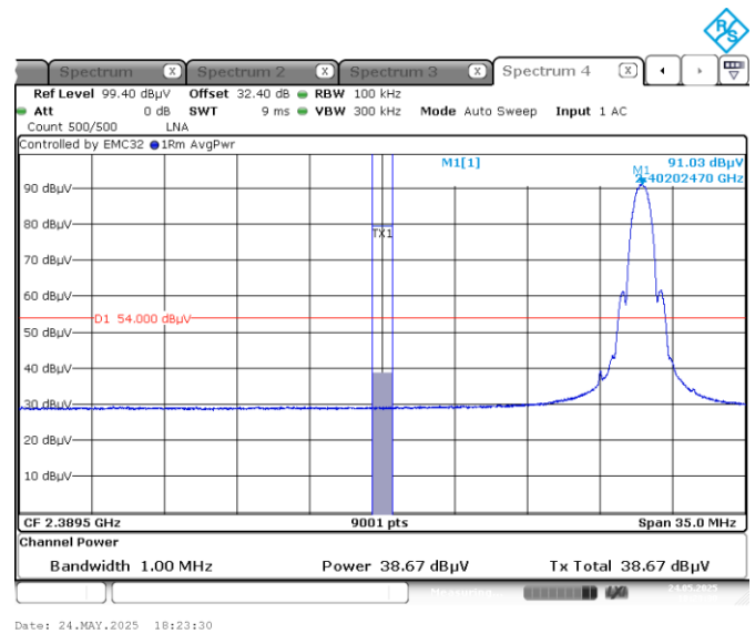
Figure 7.7-11: Band edge spurious emissions at 2390 MHz Average
