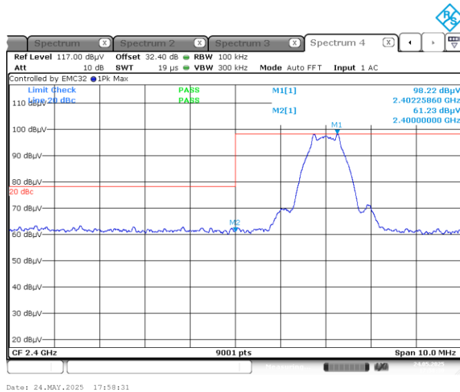
Figure 7.7-14: Non-restricted band edge emissions at 2400 MHz
