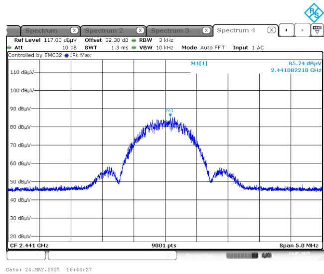
Figure 7.8-2: PSD on mid channel
