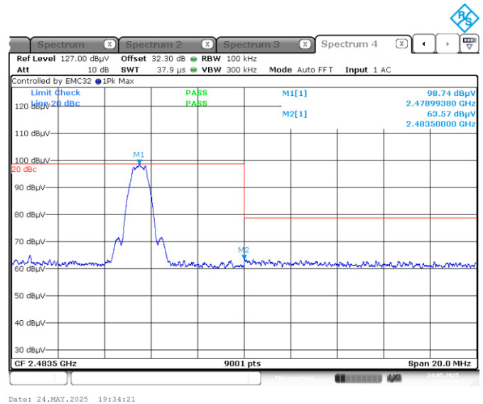
Figure 7.7-15: Non-restricted band edge emissions at 2483.5 MHz
