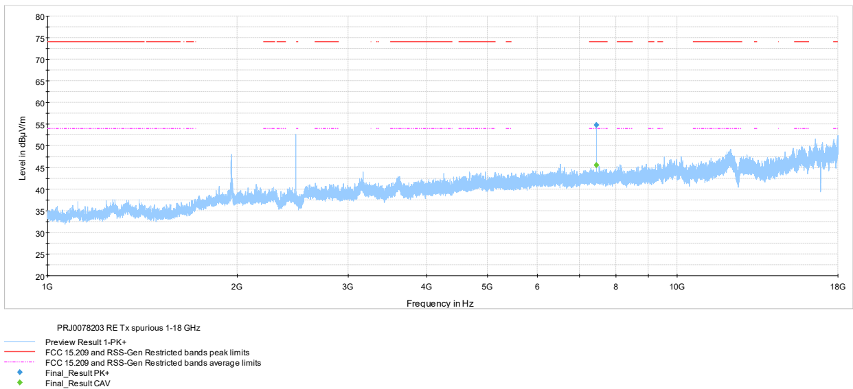
Figure 7.7-6: Radiated spurious emissions 1-18 GHz high channel
