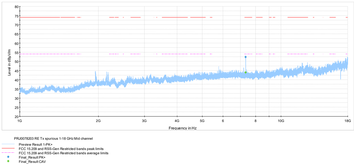
Figure 7.7-5: Radiated spurious emissions 1-18 GHz mid channel
