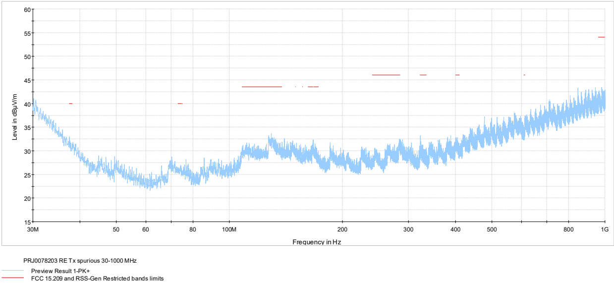
Figure 7.7-2: Radiated spurious emissions 30-1000 MHz mid channel
