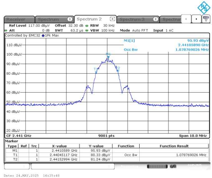
Figure 7.5-5: 99% occupied bandwidth on mid ch.
