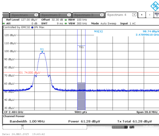
Figure 7.7-12: Band edge spurious emissions at 2483.5 MHz Peak
