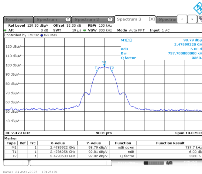
Figure 7.5-3: 6 dB bandwidth on high ch.
