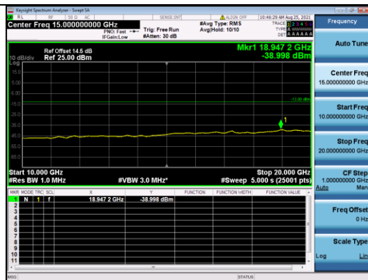
CATM1 B4-1.4M-High CH-CSE-1-QPSK-1 RB 0
