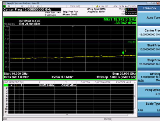
CATM1 B4-5M-High CH-CSE-1-QPSK-1 RB 0
