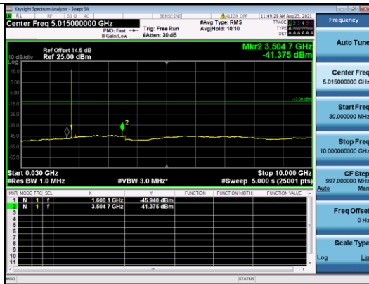
CATM1 B4-3M-High CH-CSE-2-QPSK-1 RB 0
