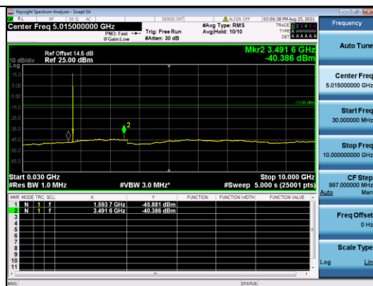
CATM1 B4-10M-High CH-CSE-2-QPSK-1 RB 0
