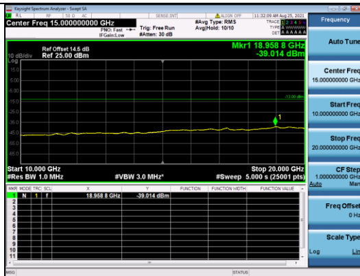
CATM1 B4-3M-Mid CH-CSE-1-QPSK-1 RB 0
