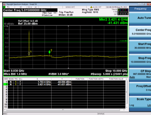
CATM1 B4-10M-Low CH-CSE-2-QPSK-1 RB 0
