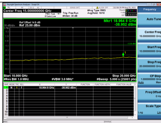
CATM1 B4-10M-High CH-CSE-1-QPSK-1 RB 0
