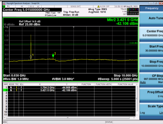
CATM1 B4-3M-Low CH-CSE-2-QPSK-1 RB 0
