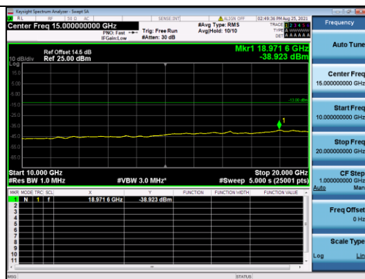
CATM1 B4-10M-Mid CH-CSE-1-QPSK-1 RB 0
