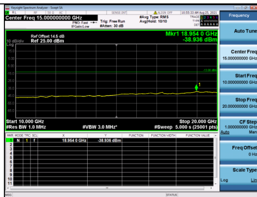
CATM1 B4-1.4M-High CH-CSE-2-QPSK-1 RB 0
