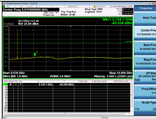
B12-5M-High CH-CSE-1-QPSK-1 RB 0
