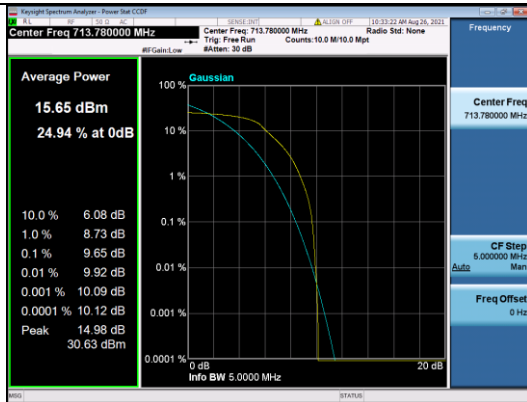
LTE CATM1 B12-3M-High CH-PAPR-QPSK
