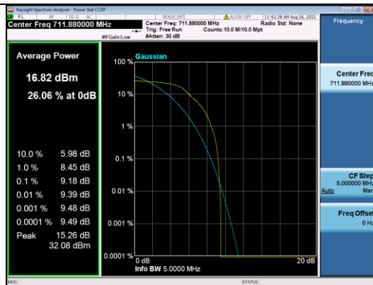
LTE CATM1 B12-5M-High CH-PAPR-QPSK
