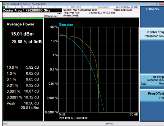
LTE CATM1 B4-15M-High CH-PAPR-QPSK
