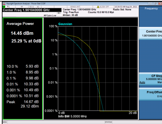
LTE CATM1 B2-10M-High CH-PAPR-QPSK
