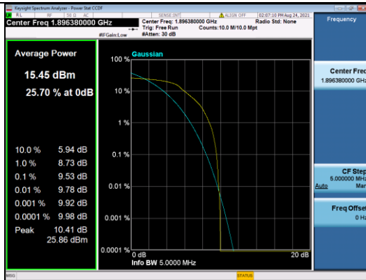
LTE CATM1 B2-15M-High CH-PAPR-QPSK
