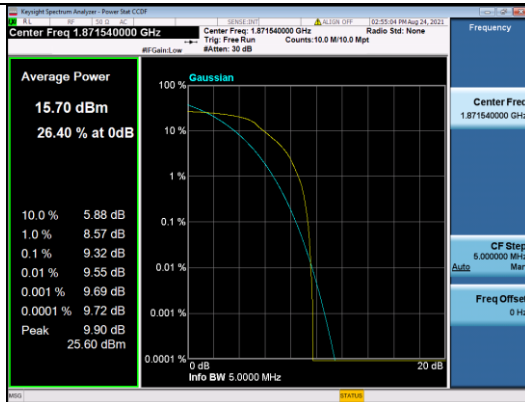
LTE CATM1 B2-20M-High CH-PAPR-QPSK
