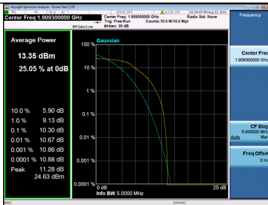
LTE CATM1 B2-1.4M-High CH-PAPR-QPSK
