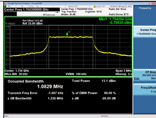
LTE CATM1 B4-1.4M-High CH-OBW-Q16
