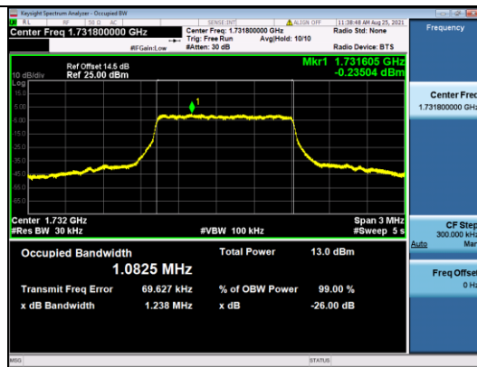
LTE CATM1 B4-3M-High CH-OBW-QPSK
