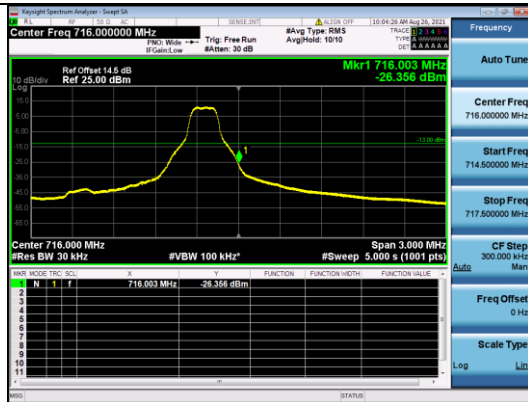
CATM1 B12-1.4M-High CH-BE-QPSK-1 RB MAX
