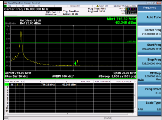
CATM1 B12-10M-High CH-BE-Q16-1 RB MAX
