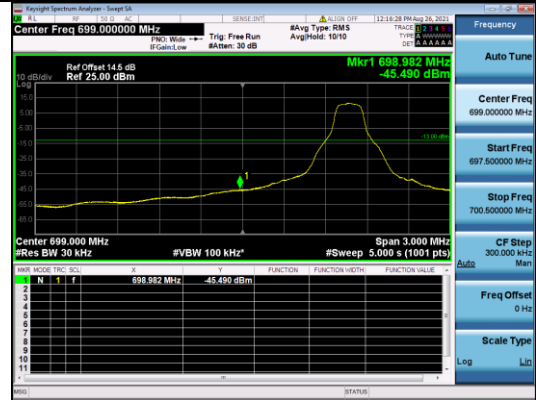
CATM1 B12-10M-Low CH-BE-Q16-Full RB 0
