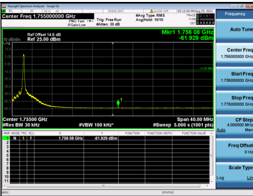
CATM1 B4-20M-High CH-BE-QPSK-Full RB 0
