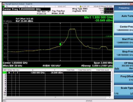
CATM1 B2-5M-Low CH-BE-QPSK-1 RB 0
