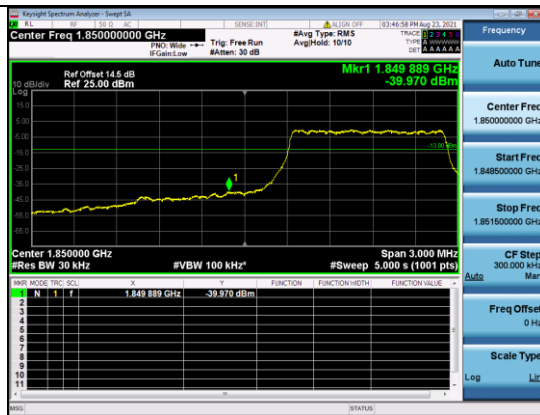
CATM1 B2-3M-Low CH-BE-QPSK-Full RB 0
