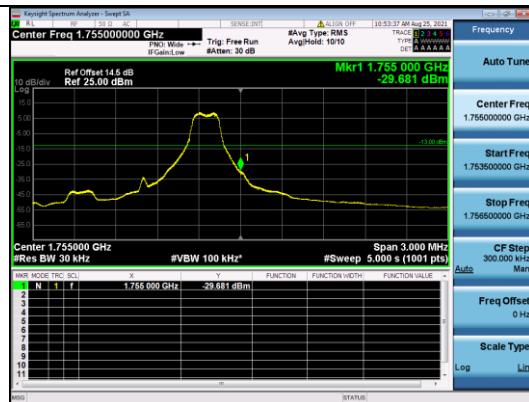
CATM1 B4-1.4M-High CH-BE-QPSK-1 RB MAX
