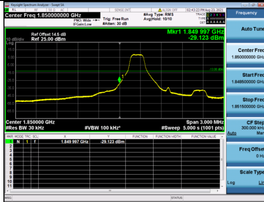
CATM1 B2-1.4M-Low CH-BE-QPSK-Full RB 0
