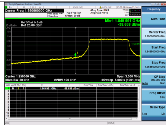
CATM1 B2-3M-Low CH-BE-Q16-Full RB 0
