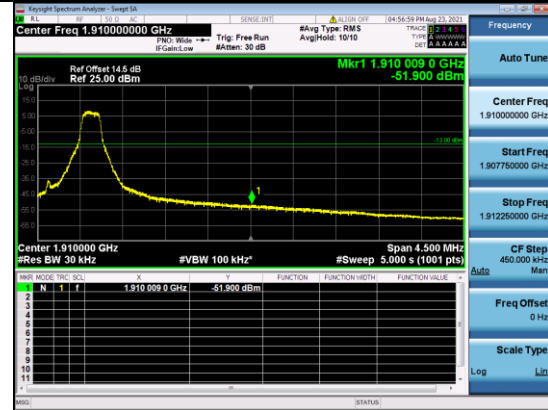
CATM1 B2-3M-High CH-BE-Q16-Full RB 0
