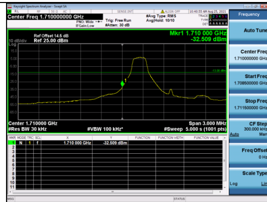
CATM1 B4-1.4M-Low CH-BE-Q16-Full RB 0
