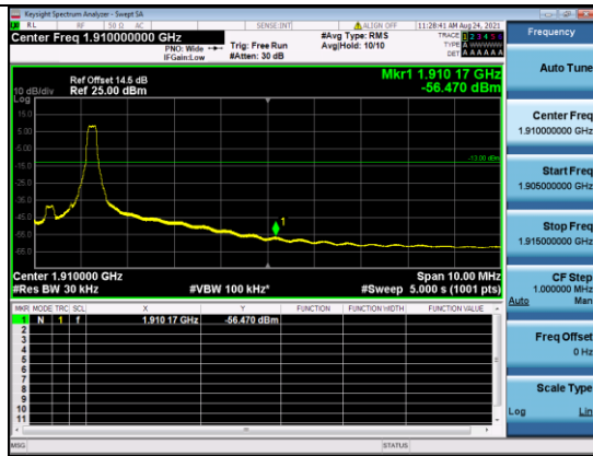
CATM1 B2-5M-High CH-BE-QPSK-Full RB 0
