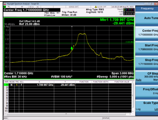
CATM1 B4-1.4M-Low CH-BE-QPSK-Full RB 0
