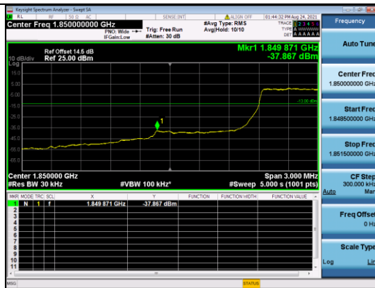
CATM1 B2-15M-Low CH-BE-QPSK-Full RB 0
