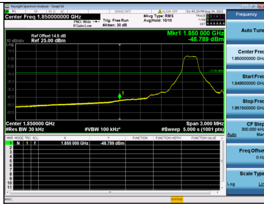
CATM1 B2-15M-Low CH-BE-QPSK-Full RB 0
