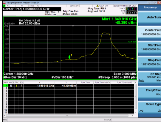
CATM1 B2-10M-Low CH-BE-QPSK-Full RB 0
