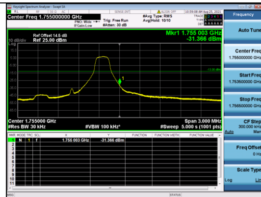
CATM1 B4-1.4M-High CH-BE-Q16-1 RB MAX
