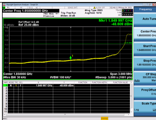
CATM1 B2-20M-Low CH-BE-QPSK-1 RB 0
