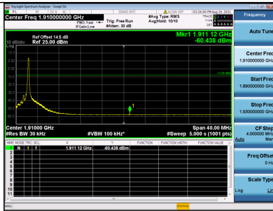
CATM1 B2-20M-High CH-BE-QPSK-Full RB 0
