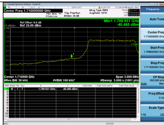
CATM1 B4-3M-Low CH-BE-QPSK-Full RB 0
