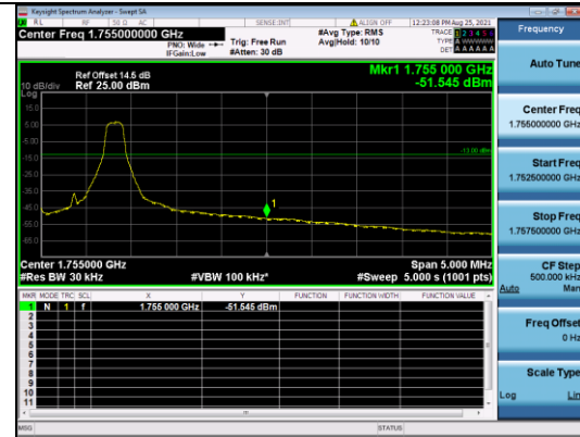
CATM1 B4-3M-High CH-BE-Q16-Full RB 0
