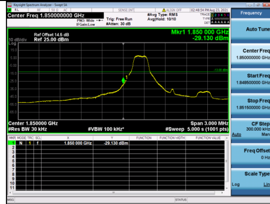
CATM1 B2-1.4M-Low CH-BE-Q16-Full RB 0
