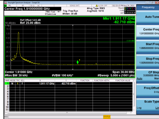
CATM1 B2-15M-High CH-BE-Q16-Full RB 0
