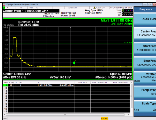
CATM1 B2-20M-High CH-BE-QPSK-Full RB 0
