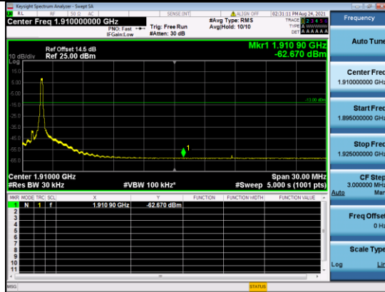
CATM1 B2-15M-High CH-BE-QPSK-Full RB 0
