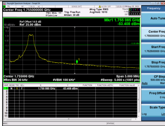
CATM1 B4-3M-High CH-BE-QPSK-Full RB 0
