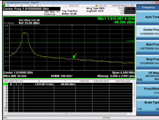
CATM1 B2-3M-High CH-BE-QPSK-Full RB 0
