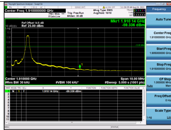
CATM1 B2-5M-High CH-BE-Q16-Full RB 0
