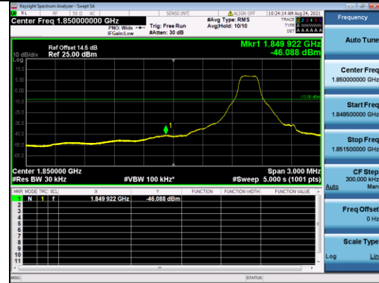
CATM1 B2-10M-Low CH-BE-Q16-Full RB 0
