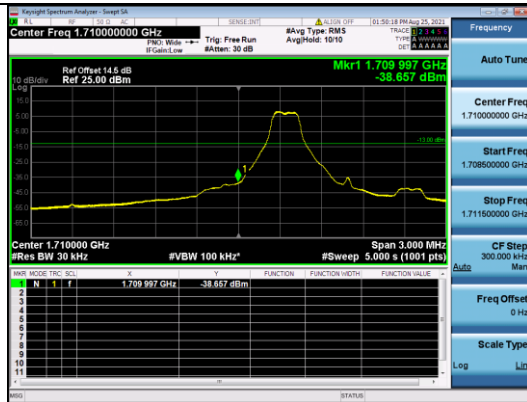
CATM1 B4-5M-Low CH-BE-QPSK-1 RB 0
