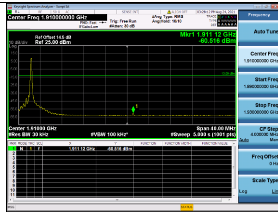
CATM1 B2-20M-High CH-BE-Q16-Full RB 0
