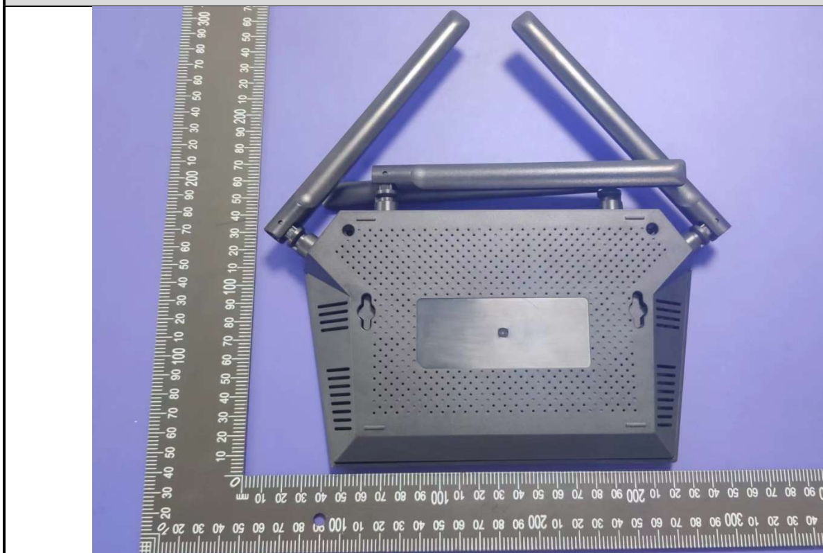
EUT4 Photo
