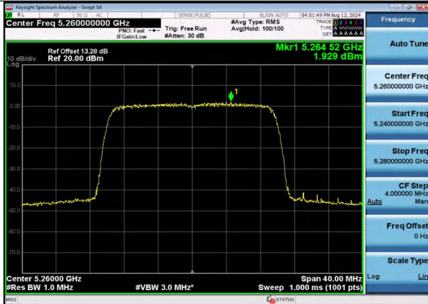
11AX20SISO-Ant1-5260-PASS
