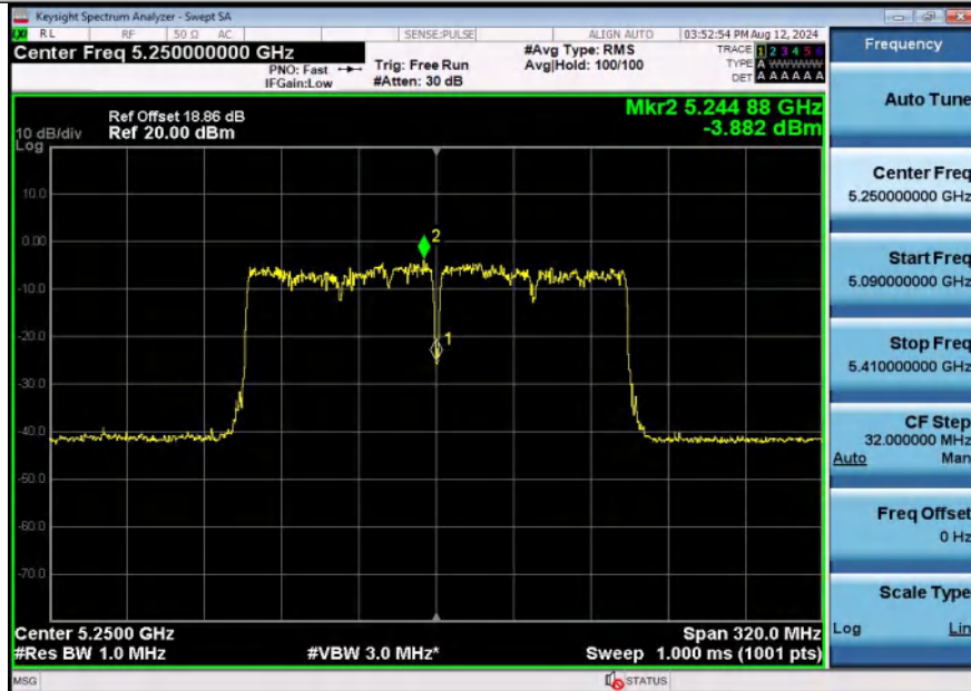
11AC160SISO-Ant1-5250_UNII-1-PASS
