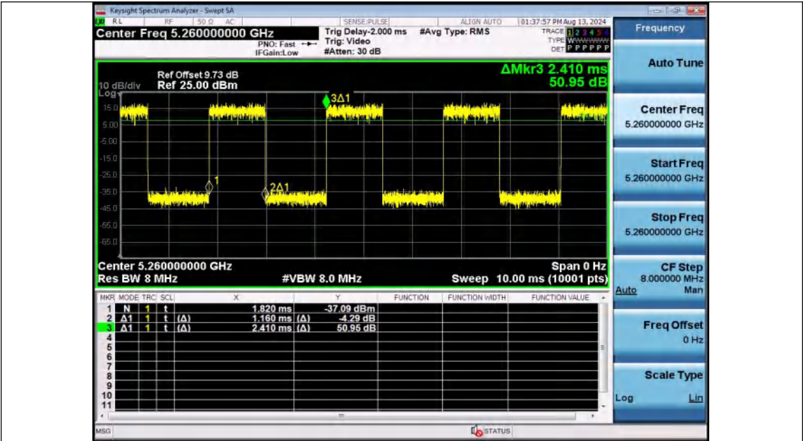
NTNV-11AC20SISO-Ant2-5260
