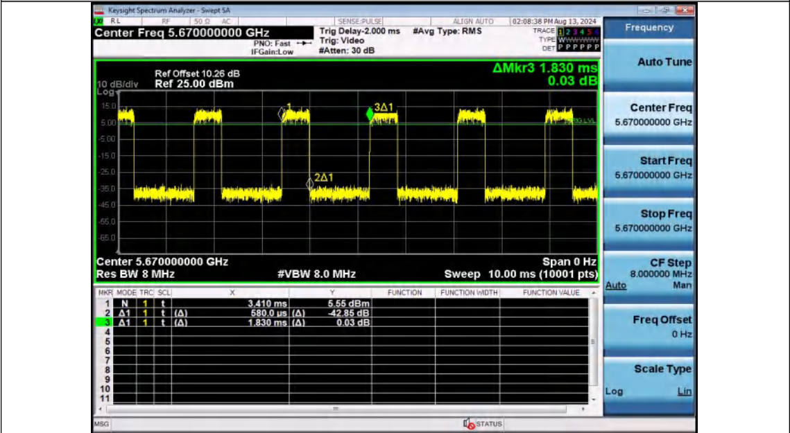
NTNV-11AC40SISO-Ant2-5670
