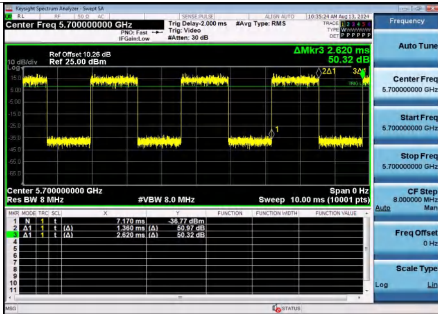
NTNV-11A-Ant2-5700
