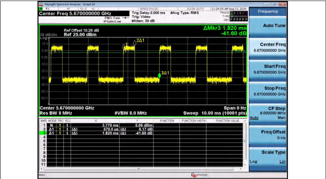
NTNV-11N40SISO-Ant2-5670
