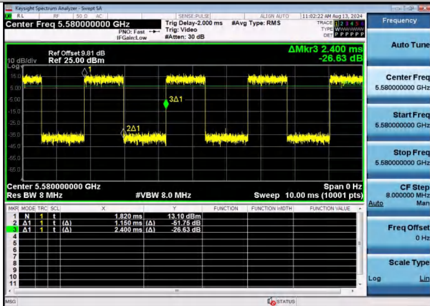
NTNV-11N20SISO-Ant2-5580
