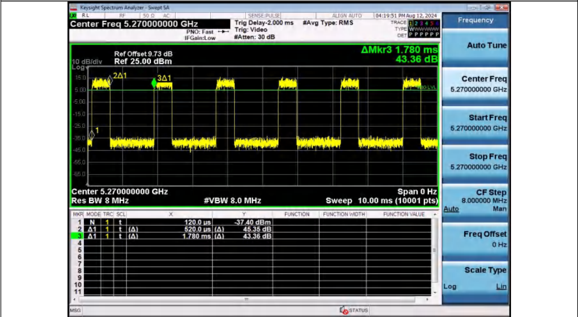
NTNV-11AX40SISO-Ant1-5270
