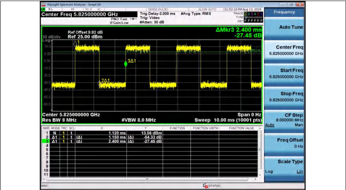
NTNV-11AC20SISO-Ant2-5825
