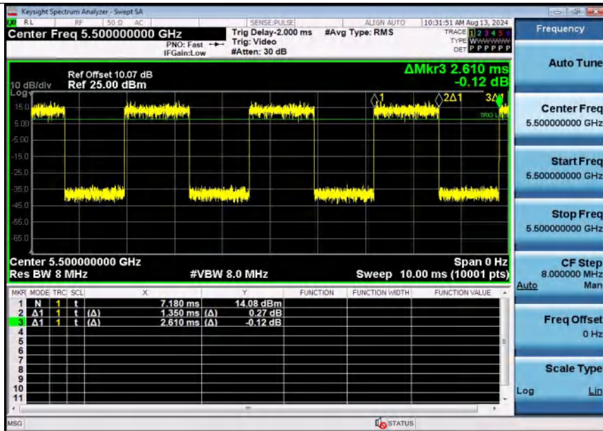
NTNV-11A-Ant2-5500
