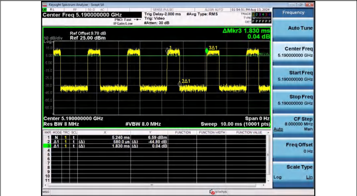
NTNV-11AC40SISO-Ant2-5190
