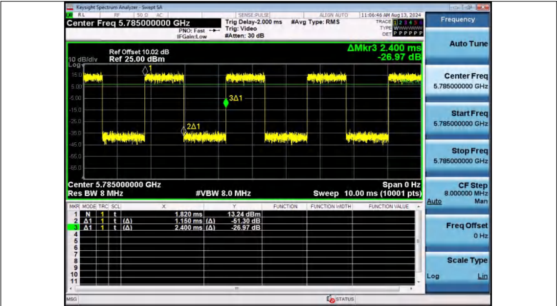
NTNV-11N20SISO-Ant2-5785
