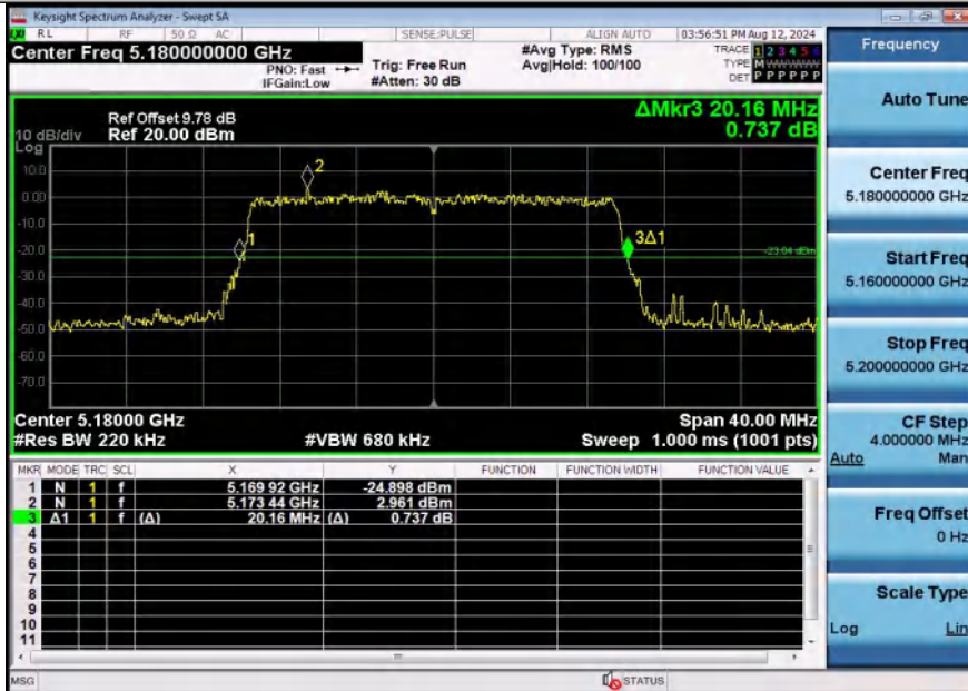
11AX20SISO-Ant1-5180
