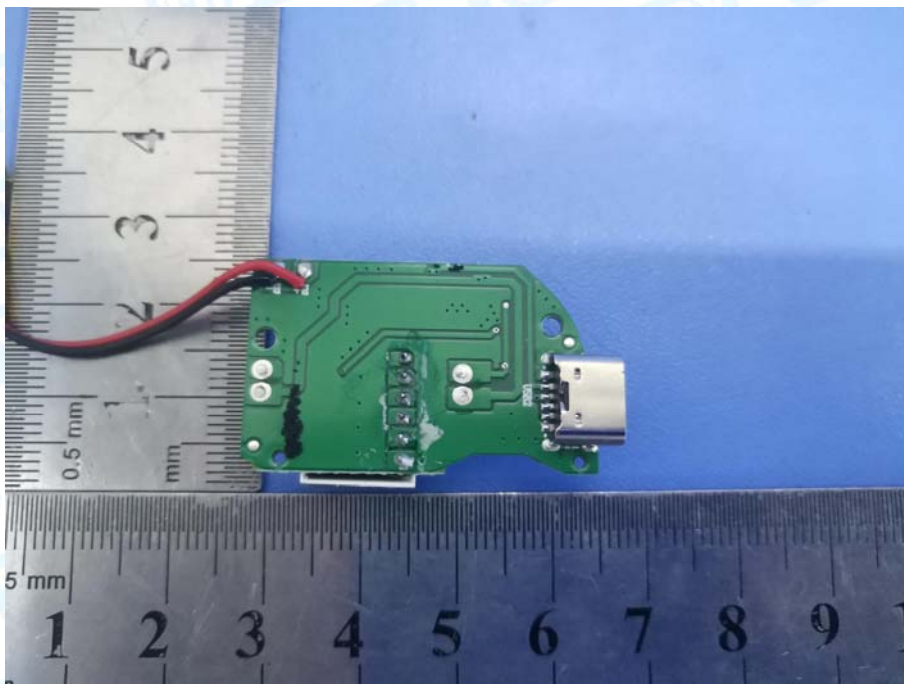
Photo 13 Internal of PCB&Battery
