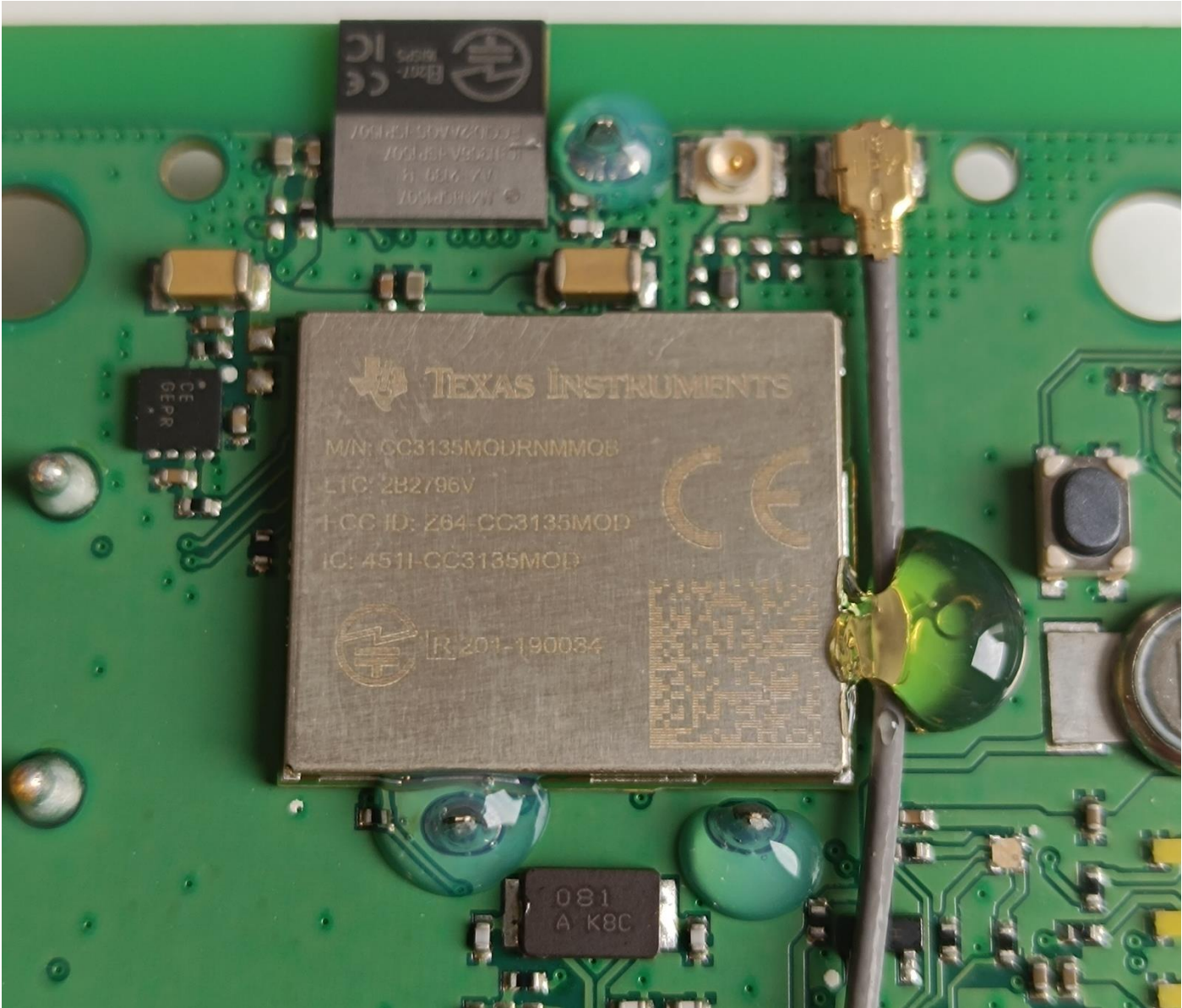
Zoomed view on Wifi Module without FCC ID Label
