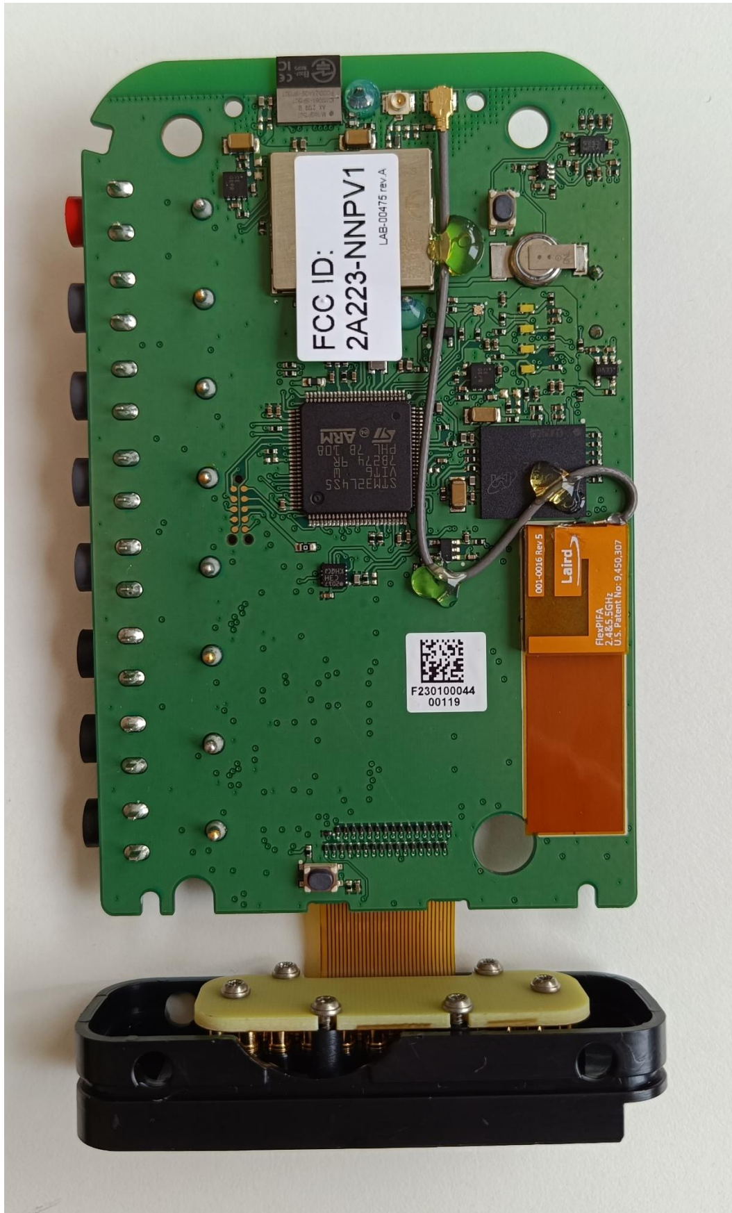
Global PCBA view with FCC ID Label
